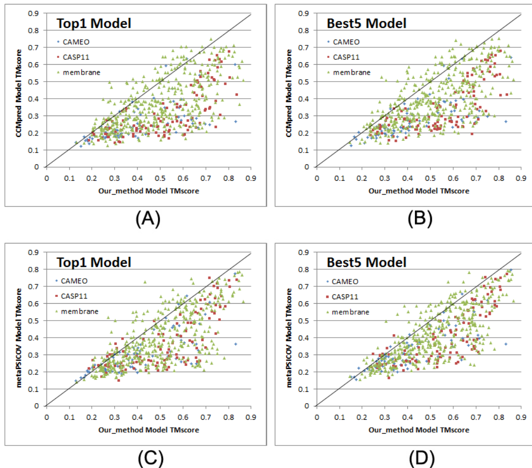
Figure 3. Quality comparison (measured by TMscore) of contact-assisted models generated by our method, CCMpred and MetaPSICOV on the 105 CASP11 targets (red square), 76 CAMEO targets (blue diamond) and 398 membrane protein targets (green triangle), respectively. (A) and (B): comparison of top 1 and the best of top 5 models between our method (X-axis) and CCMpred (Y-axis). (C) and (D): comparison of top 1 and the best of top 5 models between our method (X-axis) and MetaPSICOV (Y-axis).
