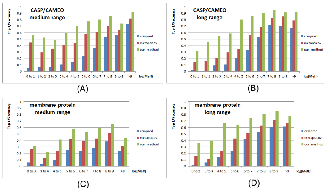
Figure 2. Top L/5 accuracy of our method (green), CCMpred (blue) and MetaPSICOV (red) with respect to the amount of homologous information measured by \ln(M_{eff}) . The accuracy on the union of
