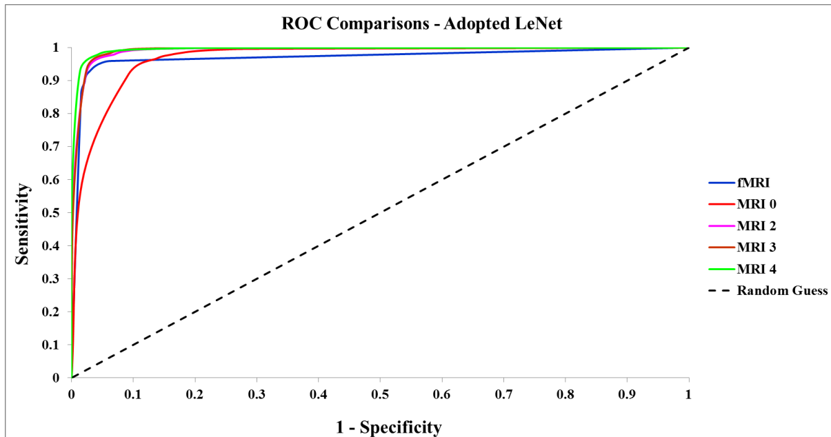
Figure 13: The averaged sensitivity and 1-specificity for five categories of classification which included the adopted LeNet models of rs-fMRI and structural MRI smoothed by four different Gaussian kernels, were used to illustrate ROCs. The comparisons of ROCs indicated that the performance of 1) each classifier 2) DeepAD pipeline was beyond random guess and tended towards the perfect binary classification.
