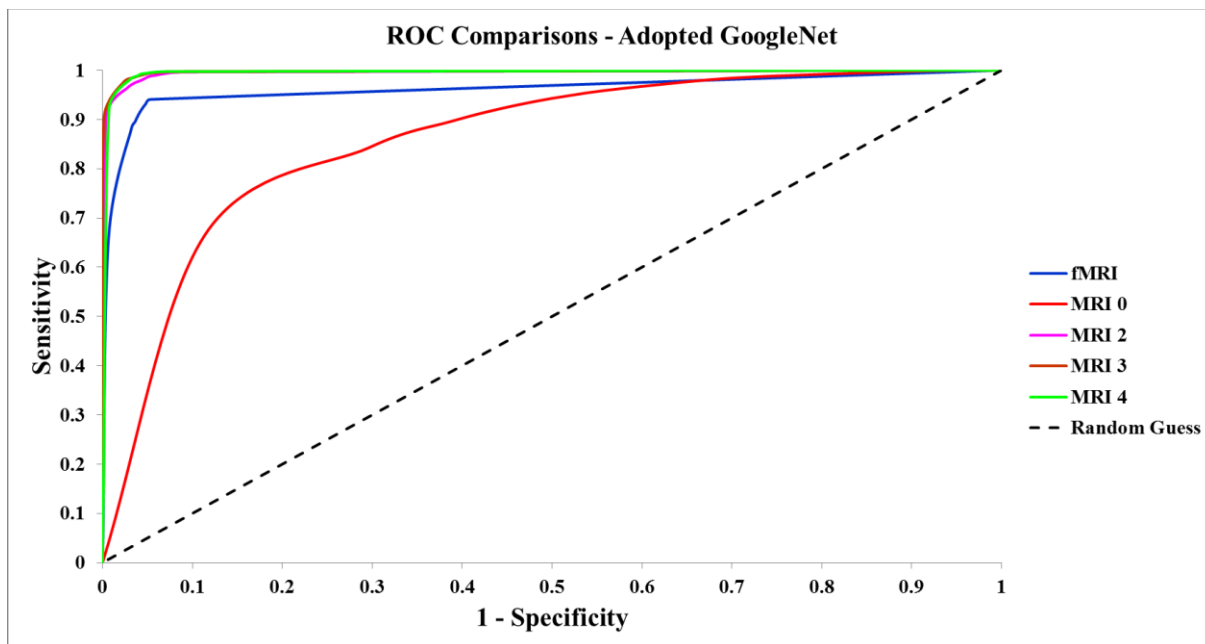
Figure 14: The ROC curves drawn for Sensitivity over 1 - Specificity illustrate the performance of the adopted GoogleNet classifiers. The MRI dataset smoothed by a Gaussian filter of 3 and 4 mm show the best performance. The MRI 2 and fMRI also indicate that the classification was very well performed. However, the MRI dataset without spatial smoothing did not compete with other classifiers.
