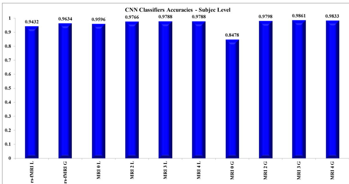
Figure 12: The averaged accuracy rates of validation (Testing) samples for 10 categories of rs-fMRI and structural MRI and adopted LeNet and GoogelNet. As seen in the figure except structural MRI dataset without smoothing, all categories resulted in very high accuracy rates.
