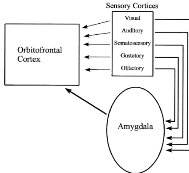
Figure 10. The orbitofrontal cortex (executive control) receives information from sensory cortices, and also from the amygdala for past events and emotions. Modified from Figure 3 of Barbas (2000).
