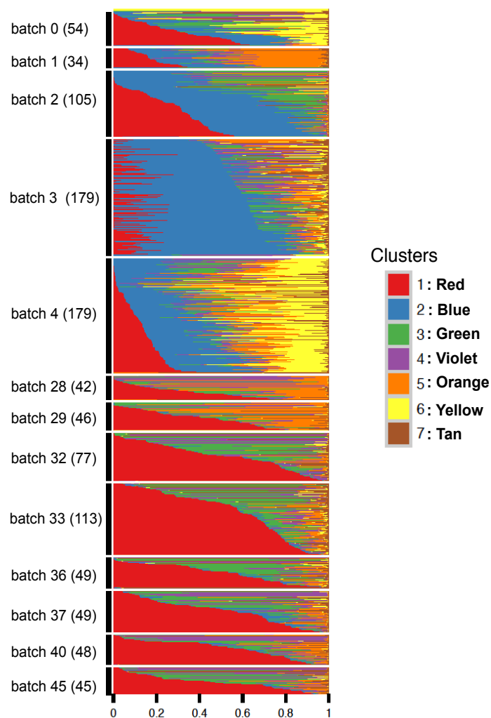
Fig 3. Structure plot of estimated membership proportions for GoM model with K = 7 clusters fit to 1,041 single cells from [22]. The samples (cells) are ordered so that samples from the same amplification batch are adjacent and within each batch, the samples are sorted by the proportional representation of the underlying clusters. In this analysis the samples do not appear to form clearly-defined clusters, with each sample being allocated membership in several “clusters”. Membership proportions are correlated with batch, and some groups of batches (e.g. 28-29; 32-45) show similar palettes. These results suggest that batch effects are likely influencing the inferred structure in these data.
