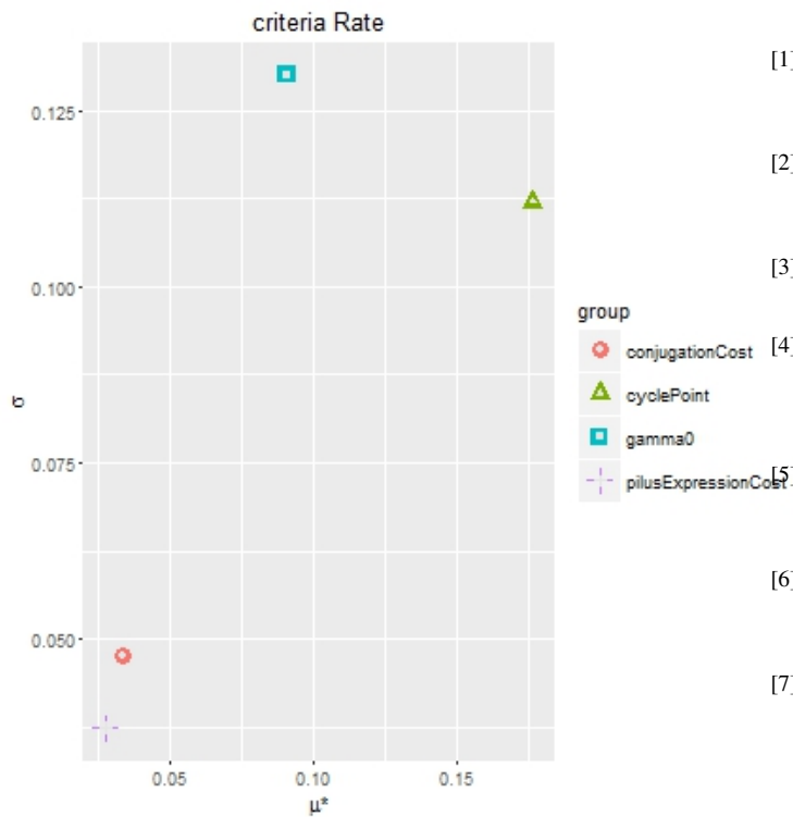
Figure 4: One of the output charts for Morris's screening method. The chart shows that the most import parameter for the Rate calibration metric is the cyclePoint followed by the gamma0.
