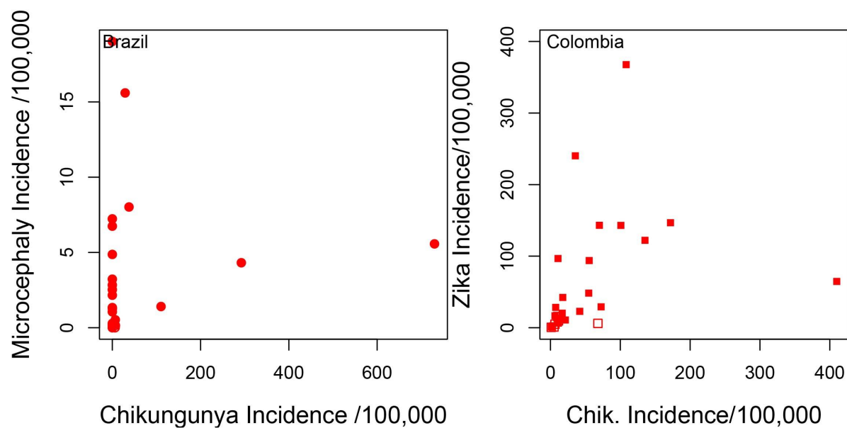
Figure 2: Correlation between Chikungunya incidence with the incidence of microcephaly in states of Brazil and the incidence of Zika in departments Colombia. There is only a weak correlation between Chikungunya and Zika incidence in Colombia ( R^2 = 0.11 , p=0.09 ), and no observable correlation in Brazil ( R^2 = 0.01 , p=0.54 ),.
