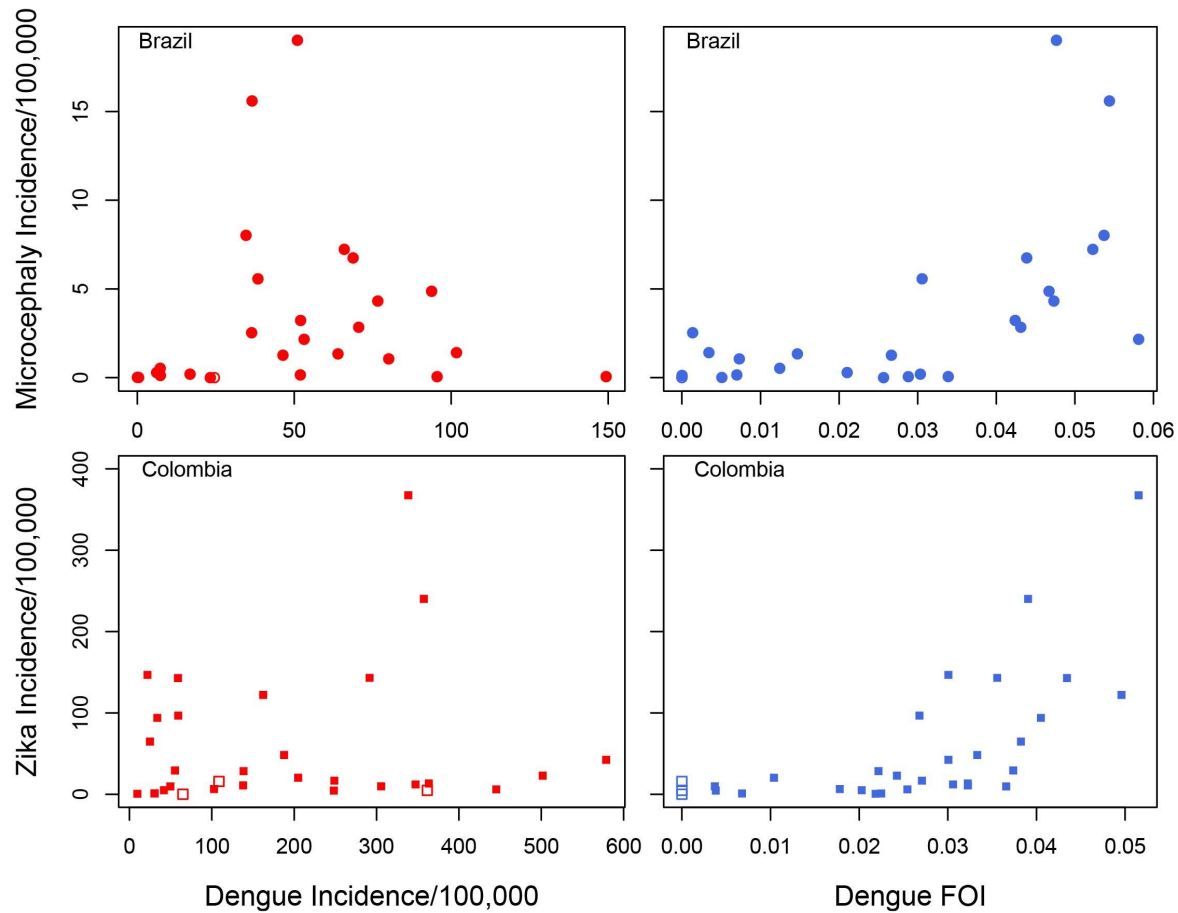
Figure 1: Correlation between dengue incidence (left) and dengue force of infection (right) with the incidence of microcephaly in states of Brazil and the incidence of Zika in continental departments Colombia. While there is no apparent correlation between the dengue incidence and either microcephaly or Zika ( R^2=6e-5 and 0.01 , respectively), a significant positive correlation is observed between the estimated force of infection and microcephaly/Zika incidence in the two countries ( R^2= 0.36 and 0.41 , respectively. p<0.001 ). Open symbols indicate states/departments where low dengue cases counts didn't allow estimation of the force of infection
