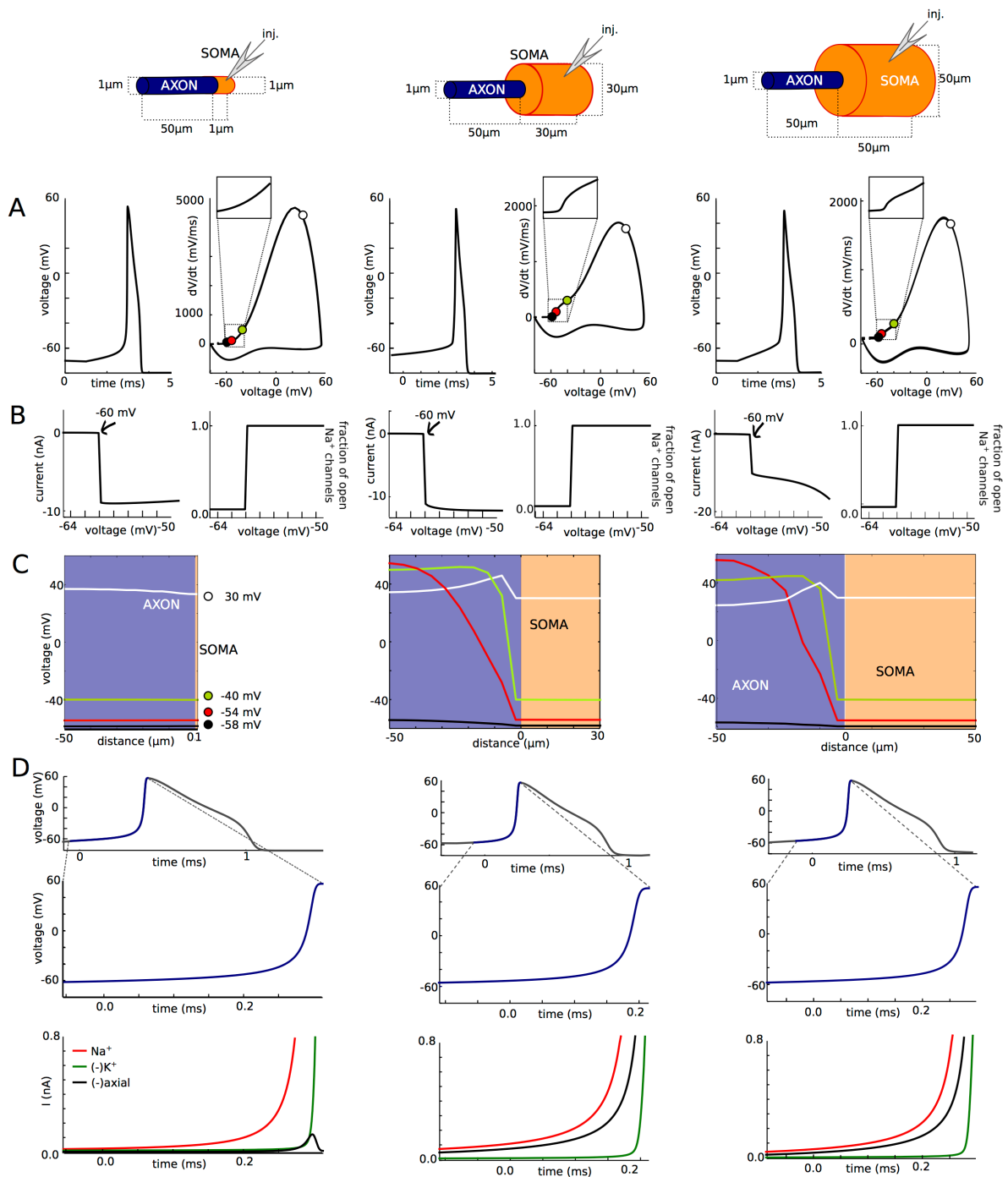
Figure 4. Influence of soma size on spike initiation. A, Somatic voltage trace and phase plot. B, Peak Na current (left) and proportion of open axonal Na channels (right) versus holding potential in somatic voltage-clamp. C, Membrane potential across the neuron at different instants near spike initiation. D, Balance of currents at initiation site (bottom) near spike initiation (top and middle: voltage trace).
