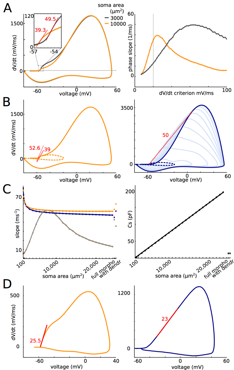
Figure 5. Somatic onset rapidness. A, Phase plot of a somatic spike with a large soma (orange, 10,000 \mu\text{m}^2 ) and a small soma (gray, 3,000 \mu\text{m}^2 ). The phase plot is linear (corresponding to locally constant phase slope) around dV/dt = 25 \text{ mV/ms} in the former case and around 60 \text{ mV/ms} in the latter case. Maximum phase slope is similar in both cases ( 39.3 and 49.5 \text{ ms}^{-1} ). B, Left: phase plot for a large soma ( 10,000 \mu\text{m}^2 ). The presence of somatic Na channels slightly decreases onset rapidness (orange, slope: 39 \text{ ms}^{-1} ). Without them, onset rapidness is 52.6 \text{ ms}^{-1} . Right: phase plots at different points along the axon (dotted blue: soma; dark blue: distal end; light blue: intermediate axonal positions). The prediction of somatic onset rapidness based on resistive coupling is the maximum slope of a tangent to the phase plot intersecting the spike initiation point, which gives 50 \text{ ms}^{-1} at the distal end (red line). C, Left: Somatic onset rapidness (orange) and prediction from axonal phase plots (blue) as a function of soma area for the simple model. The morphologically realistic model and the simple model with a dendrite are also shown on the right. Grey: somatic phase slope at 20 \text{ mV/ms} . Right: For comparison, total somatic capacitance is shown as a function of soma area. D, Somatic (left) and axonal (right) phase plots of a spike digitized from Yu et al. (2008). Maximum phase slopes are similar.
