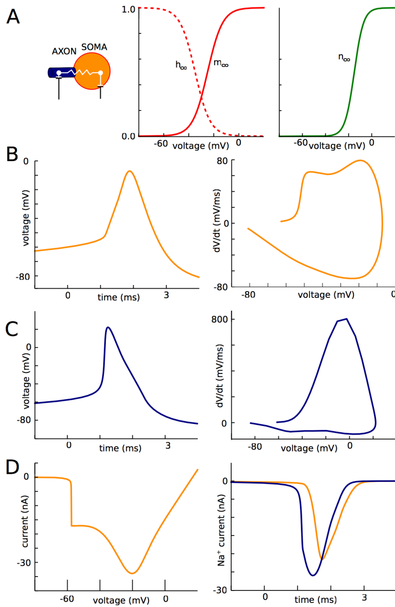
Figure 7. Two-compartment model. A, Equilibrium values of the gating variables for the Na (left) and K (right) channels. B, Voltage trace (left) and phase plot (right) of a somatic spike. C, Voltage trace (left) and phase plot (right) of an AIS spike. D, Left: Peak current recorded in somatic voltage-clamp as a function of holding voltage. Right: Na^+ current in the AIS (blue) and soma (orange) during a spike in current-clamp.
