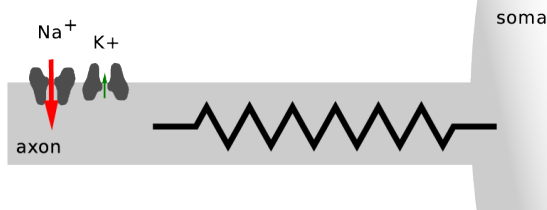
Figure 1. Theories of spike initiation. A, Standard account of spike initiation: spikes results from the interplay between Na current and K current flowing through the membrane at the initiation site. B, Top: The isopotential Hodgkin-Huxley model produces spikes with smooth onset (left), exhibiting a gradual increase in dV/dt as a function of membrane potential V (right: onset rapidness measured as the slope at 20 \text{ mV/ms} = 5.6 \text{ ms}^{-1} ). Bottom: cortical neurons have somatic spikes with sharp onsets (left), with steep increase in dV/dt as a function of V (onset rapidness: 28.8 \text{ ms}^{-1} ; human cortical data from Testa et al. (2014)). C, Backpropagation hypothesis: spikes are initiated in the axon according to the standard account, then get
