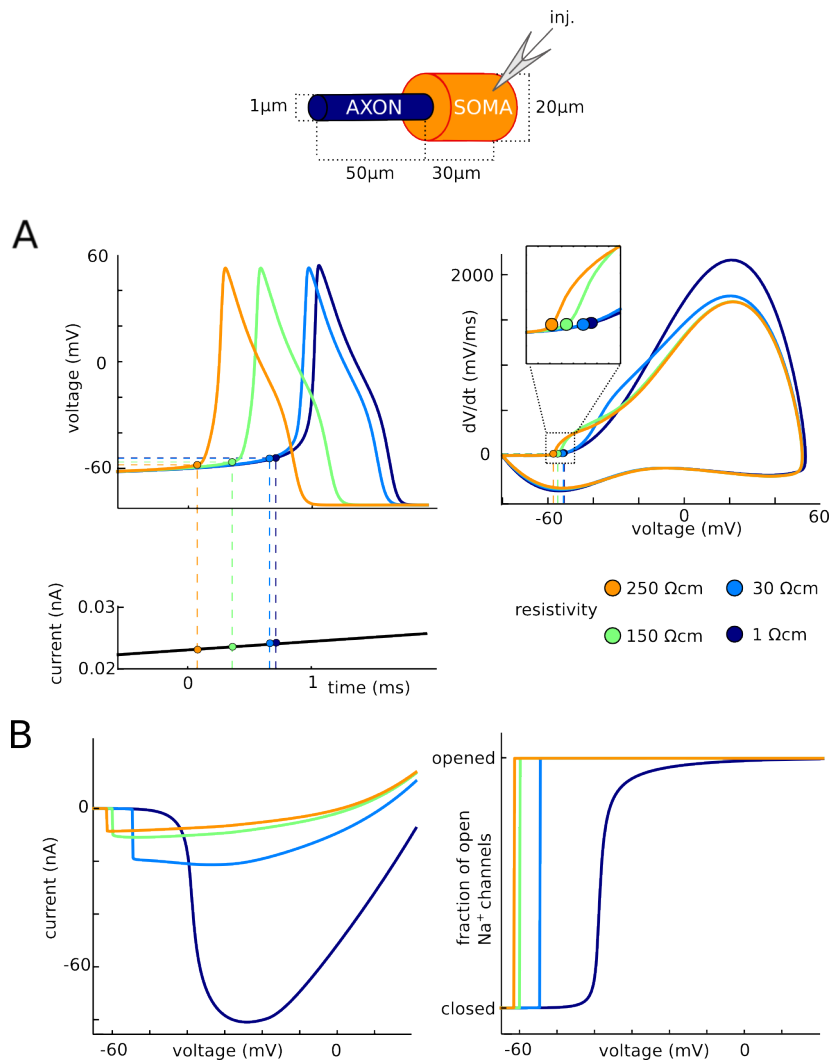
Figure 3. Impact of intracellular resistivity R_i on excitability. A, Spikes are triggered by a slow current ramp, for different values of R_i between 1 \Omega\text{cm} and 250 \Omega\text{cm} (green: original value). The neuron is more excitable for larger values of R_i . B, Current vs. somatic voltage in somatic voltage-clamp (as in Fig. 2B) and fraction of open \text{Na}^+ channels vs. somatic voltage, for different values of R_i .
