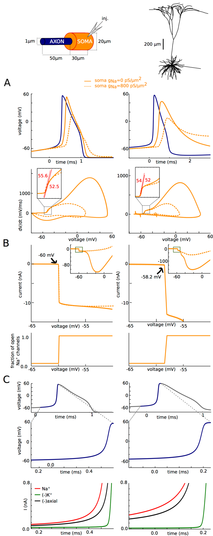
Figure 2. Spike initiation in multicompartmental models. Left: model with simplified soma-axon geometry. Right: cortical pyramidal cell model with morphological reconstruction. A, Top:
