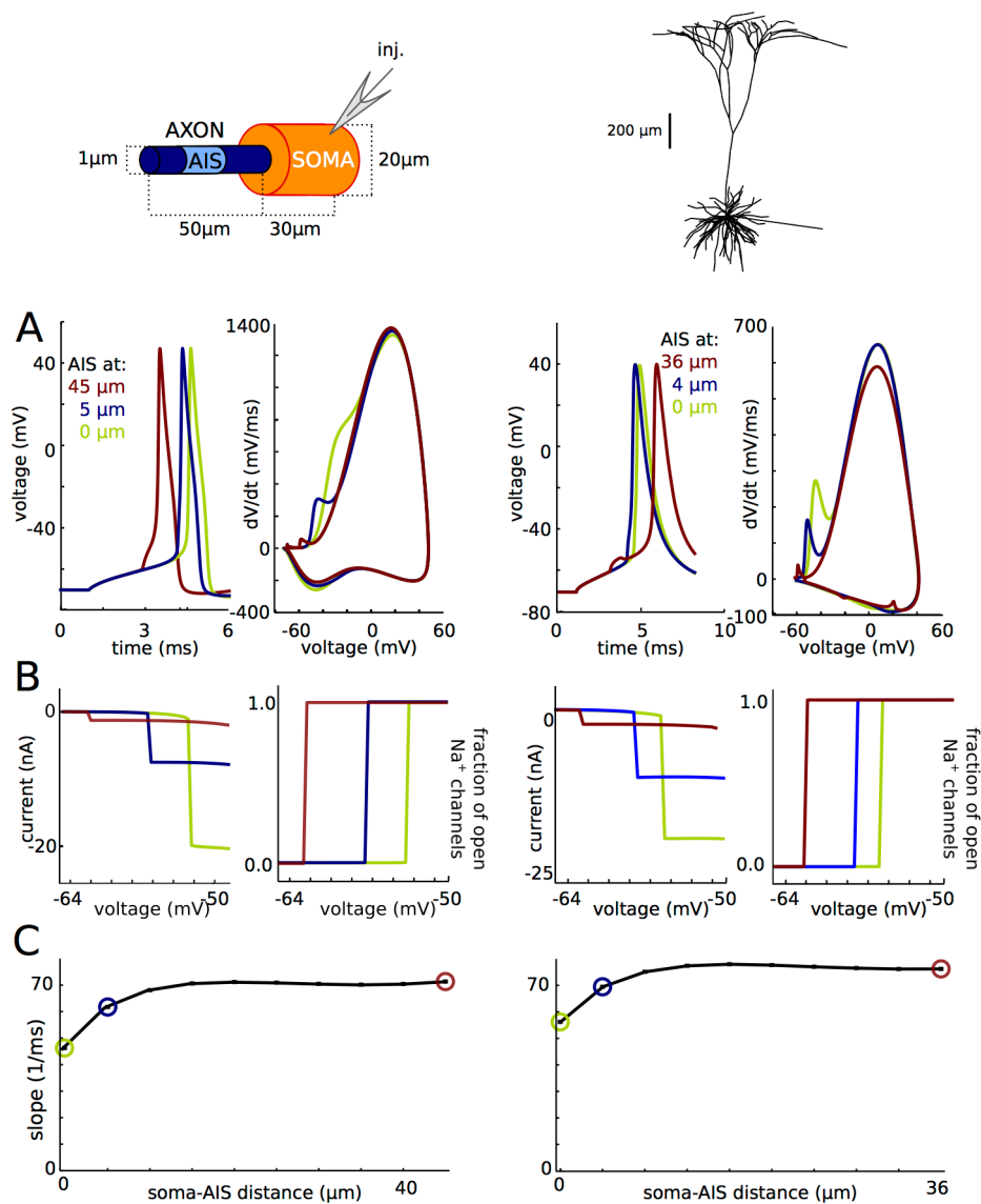
Figure 6. Active backpropagation is not necessary for sharp initiation. Left: model with simplified soma-axon geometry. Right: cortical pyramidal cell model with morphological reconstruction. A, Axonal Na channels are moved to a single axonal location (3 different locations shown). Left: voltage traces; right: phase plots. B, Peak Na current (left) and proportion of open axonal Na channels (right) versus holding potential in somatic voltage-clamp. C, Onset rapidness as a function of AIS position.
