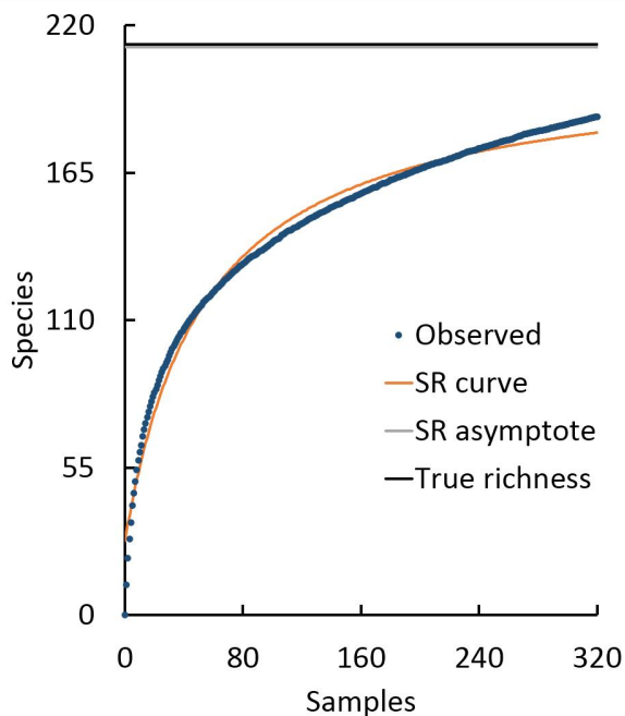
Fig. 4 – Accumulation curve for spider sampling in Gerês (Portugal) and the result of searching for the best fitting asymptotic formula using symbolic regression (SR).
