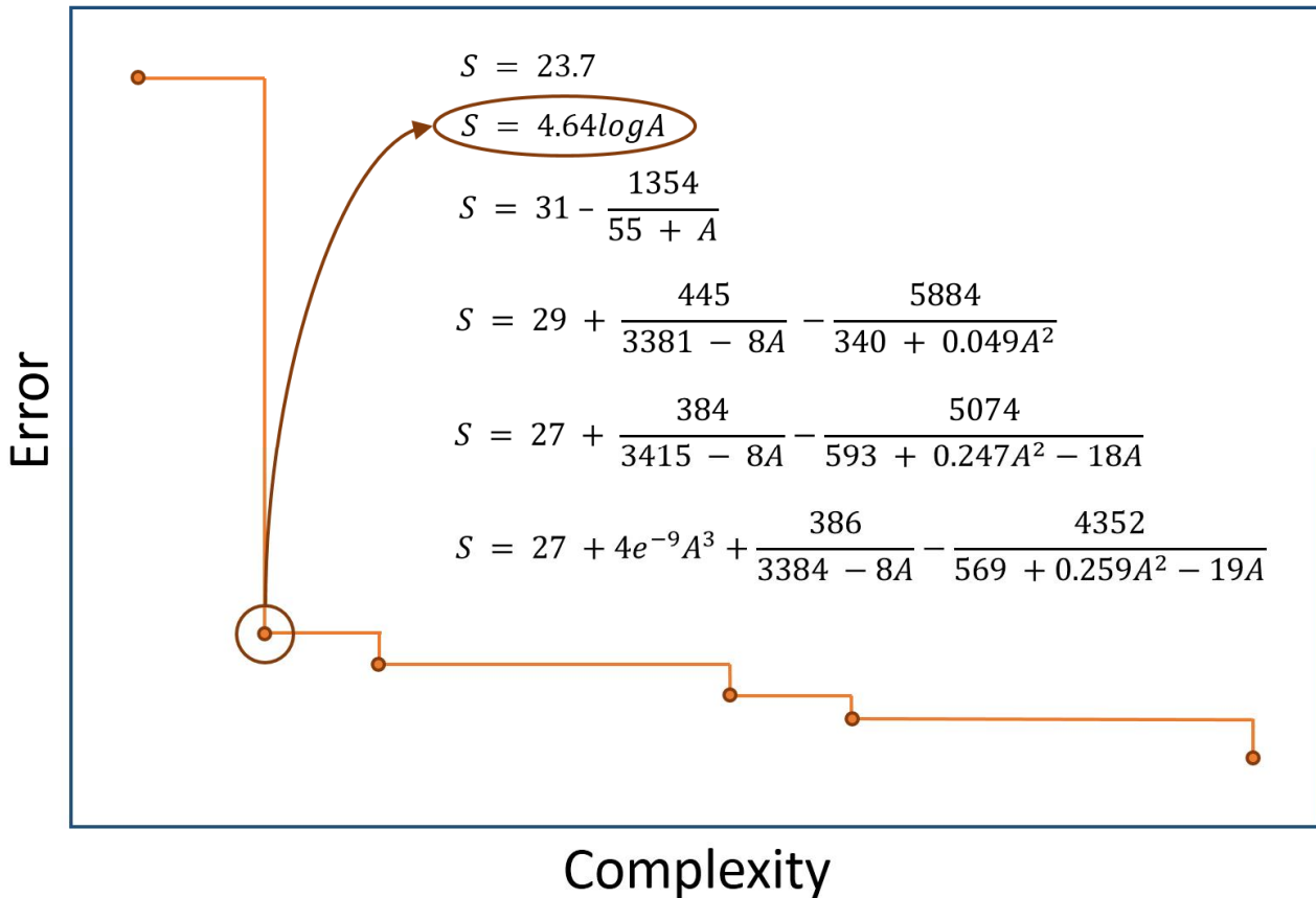
Fig 2. – Example of a Pareto front depicting error vs. complexity in the case of a symbolic regression search of the best species–area relationship for native spiders in the Azores (Portugal). The second formula is clearly the most promising, with both high accuracy (low error) and low complexity.
