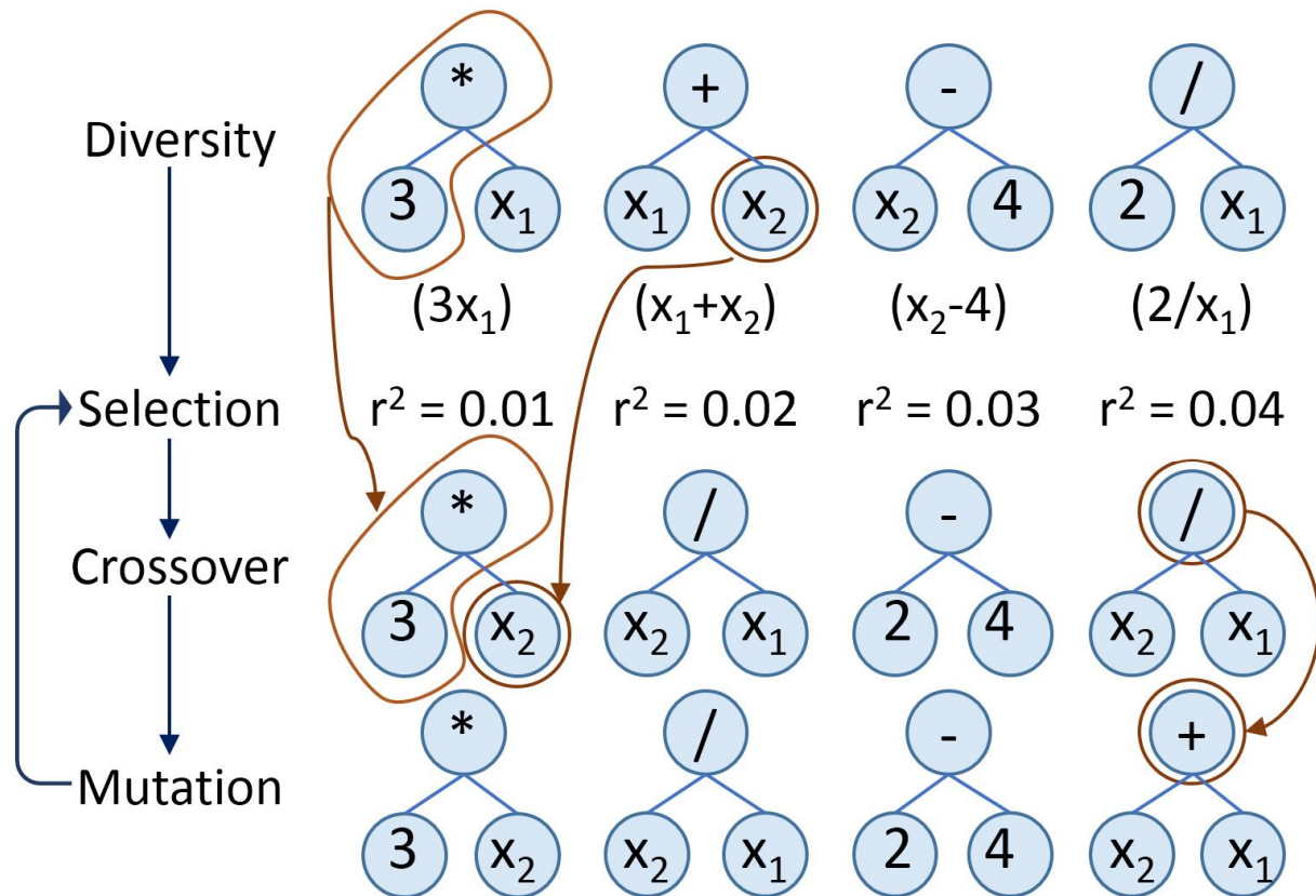
Fig. 1 – Schematic representation of the symbolic regression workflow. The basic representation is a parse-tree where building blocks such as variables (in this case: x_1 , x_2 ), parameters (integers or real numbers) and operators (e.g. + , - , \times , \div ) are connected forming functions (in parenthesis under the first line of trees). Initial equations are generated by randomly linking different building blocks. Equations are combined through crossover, giving rise to new equations with characteristics from both parents (arrows linking the first and second rows of trees). Equations with better fitness (e.g. r^2 ) have higher probabilities of recombining. To avoid loss of variability, a mutation step is added after crossover (arrows linking the second and third rows of trees). After multiple generations, evolution stops and a set of free-form equations best reflecting the input data is found.
