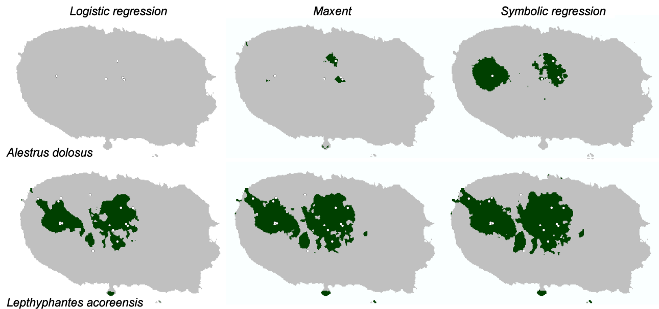
Fig. 3 – Observed locations (white dots) and predicted distribution (dark areas) of two endemic arthropod species in the island of Terceira (Azores, Portugal) using three different modelling methods.
