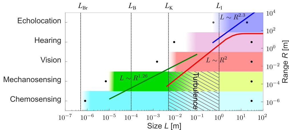
Figure 4: Upper and lower body size limits and ranges for different senses. Dots denote the largest and smallest sizes known to employ a given sense, and shaded rectangles show the theoretical estimates of the size range in which a sense is expected to work. Green, red, and blue curves show the theoretical scaling of sensing range with size for mechanosensing, vision, and echolocation, respectively.
