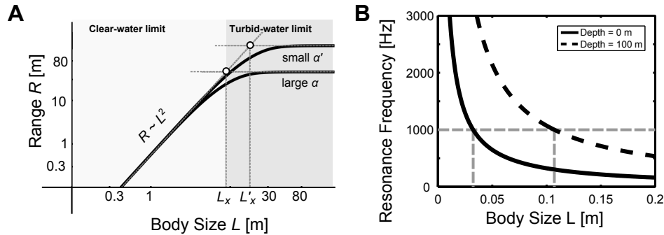
Figure 3: A: Visual sensing range scales with body size, L , as R \sim L^2 in the clear-water limit ( L \ll L_x ) and as R \sim \text{constant} in the turbid-water limit ( L \gg L_x ). Parameters are K = 0.025 , C_0 = 0.3 , C_{\text{th,min}} = 0.05 (adopted from [43]), \alpha = 0.04 \text{ m}^{-1} [69] ( \alpha' = 0.01 \text{ m}^{-1} for comparison) and a = 1 : 30 . B: Relationship of body size and resonance frequency based on Equation (7) and using a swim bladder size r_b = L/10 for an individual at the surface (solid curve) and at 100 m depth (dashed curve). The dashed (grey) horizontal line indicates 1 kHz, below which most sounds generated by marine life are found.
