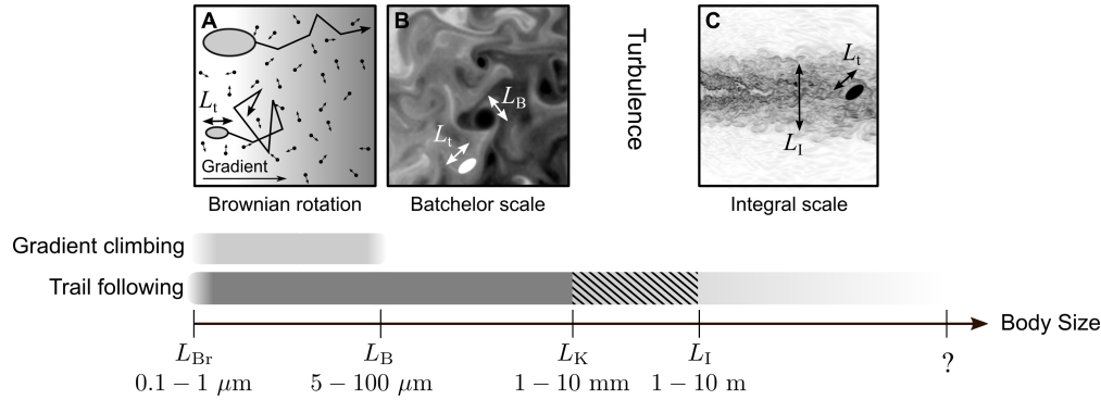
Figure 2: Body sizes over which chemosensing can be used effectively. A schematic illustration of Brownian rotation (A), Batchelor scale (B), and integral scale (C) is included at the top.
