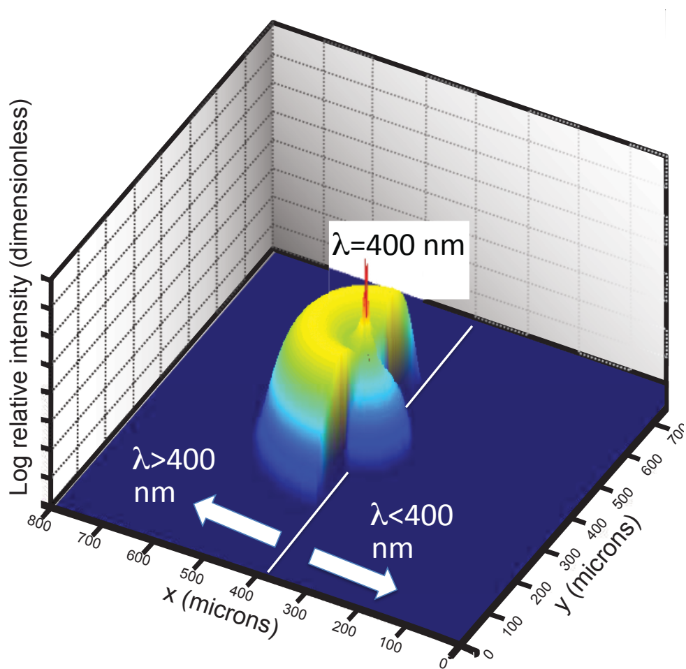
Figure S4. Chromatic PSF for 400-nm best-focus, semi-annular pupil.
