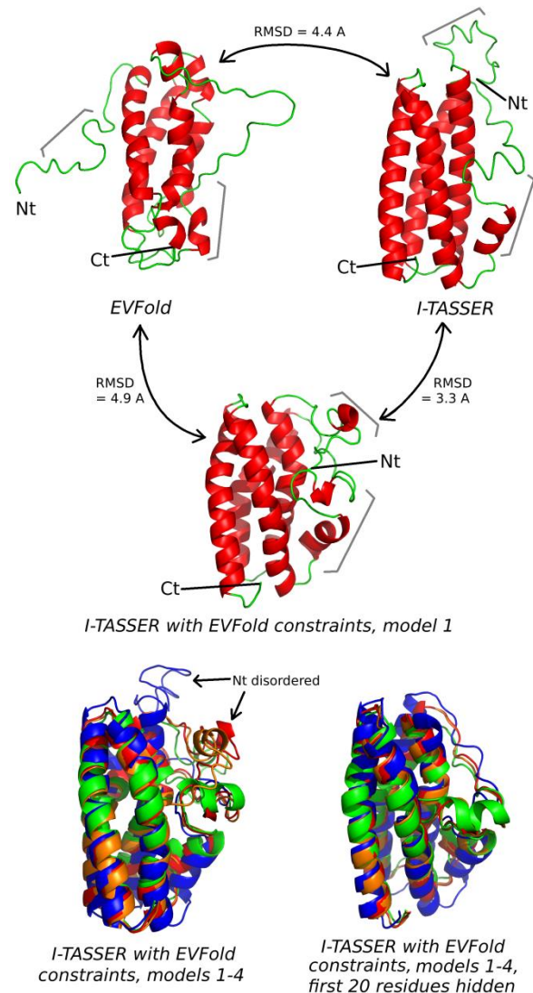
Figure 2. Models of CopM produced by EVFold (top left), I-TASSER (top right), and I-TASSER supplemented with EVFold-derived restraints (middle, first model only; and bottom, four best models, full on the left and without the first 20 residues on the right, all displayed individually in Fig. 3). All shown structures are aligned in space. Gray brackets point at the two predicted disordered regions. Black arrows in the bottom left point at the two main conformations modeled for the N-terminal region. Figures rendered with PyMOL. 16
