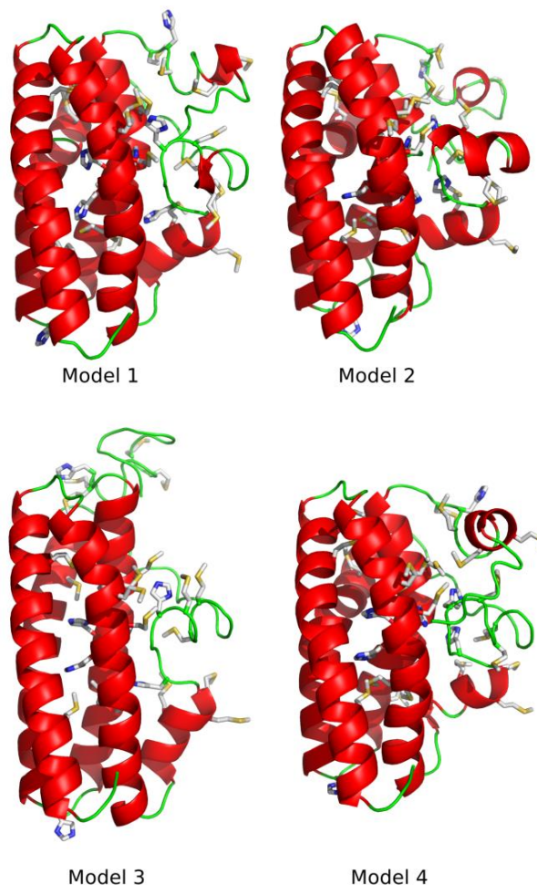
Figure 3. The four top models produced by combining the contacts computed by EVFold with homology modeling by I-TASSER. Histidine and methionine residues are rendered as sticks with standard color codes for heavy atoms.
