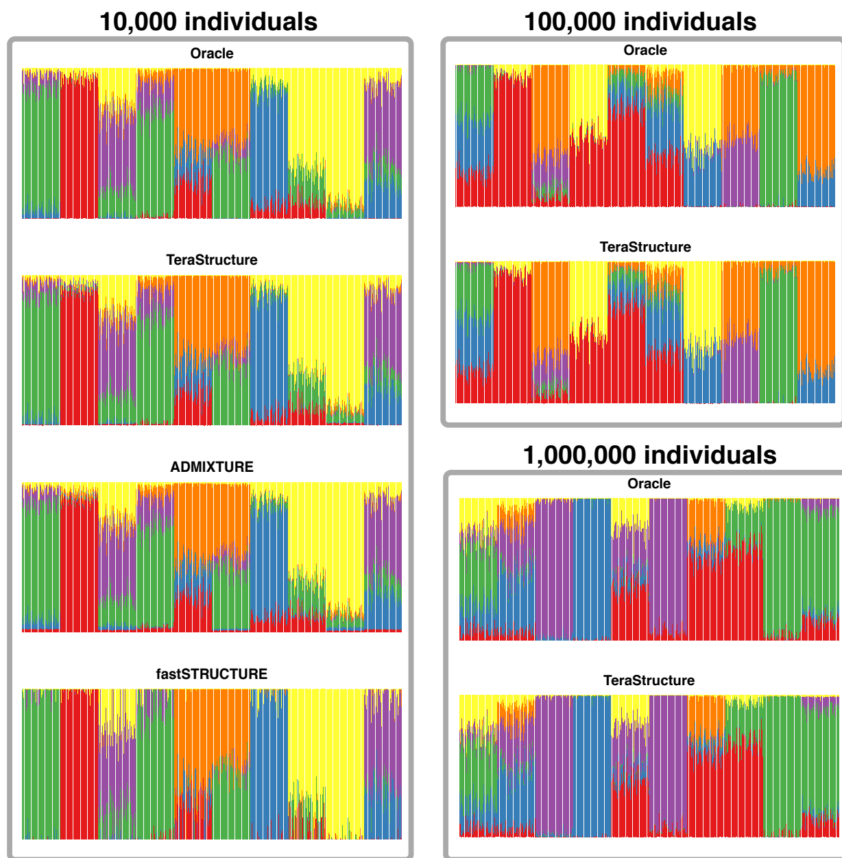
Figure 2: TeraStructure recovers the ground truth per-individual population proportions on the synthetic data sets generated via Scenario A. Each panel shows a visualization of the ground truth \theta_i^* and the inferred E[\theta_i|\hat{\theta}_i] for all individuals in a data set. The current state-of-the-art algorithms cannot complete their analyses of 100,000 and 1,000,000 individuals. TeraStructure is able to analyze data of this size and gives highly accurate estimates.
