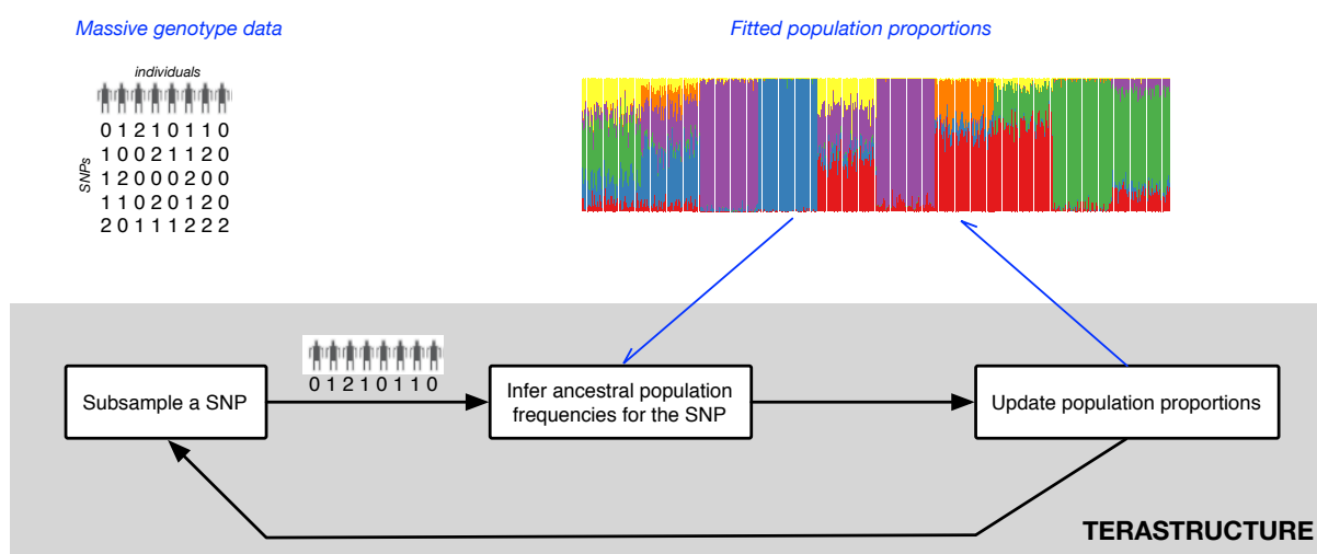
Figure 1: A schematic diagram of TeraStructure, stochastic variational inference for the Pritchard-Stephens-Donnelly (PSD) model. The algorithm maintains an estimate of the latent population proportions for each individual. At each iteration it samples SNP measurements from the large database, infers the per-population frequencies for that SNP, and updates its idea of the population proportions. This is much more efficient than algorithms that must iterate across all SNPs at each iteration.
