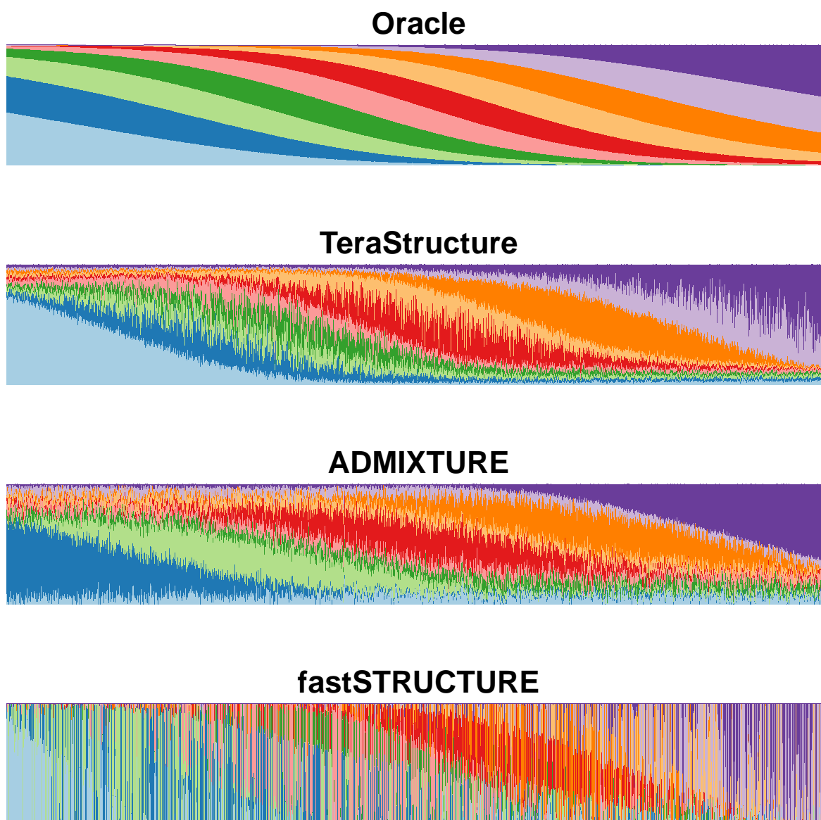
Figure 3: TeraStructure is the most accurate method for Scenario B simulations. The top panel shows the ground truth \theta_i^* , where each individual's proportions are a function of their position, e.g. the left most individual's proportions are dominated by the two blue ancestral populations while the right most individual's proportions are dominated by the two purple ancestral populations. A quantitative measure of the accuracies can be found in Table S2.
