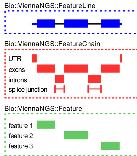
Figure 3: Schematic representation of genomic interval classes in terms of their corresponding feature annotation. Simple intervals (“features”) are characterized by Bio::ViennaNGS::Feature objects (bottom box). At the next level, Bio::ViennaNGS::FeatureChain bundles these, thereby maintaining individual annotation chains for e.g. UTRs, exons, introns, splice junctions, etc. (middle box). The topmost level is given by Bio::ViennaNGS::FeatureLine objects, representing individual transcripts.
