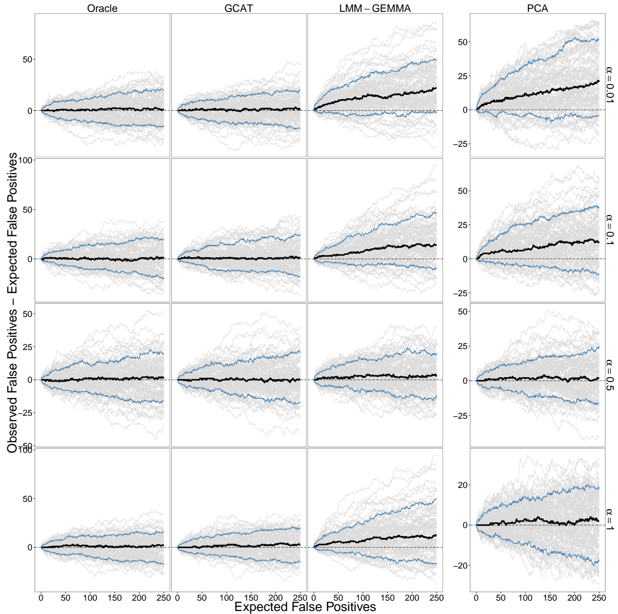
Figure S1: Performance of association tests on 100 simulated studies based off the PSD model of structure for various \alpha comparing the Oracle, GCAT (proposed), LMM (GEMMA), and PCA tests. The variance contributions to the trait are genetic=5%, environmental=5%, and noise=90%. The remaining details are equivalent to Figure 2.
