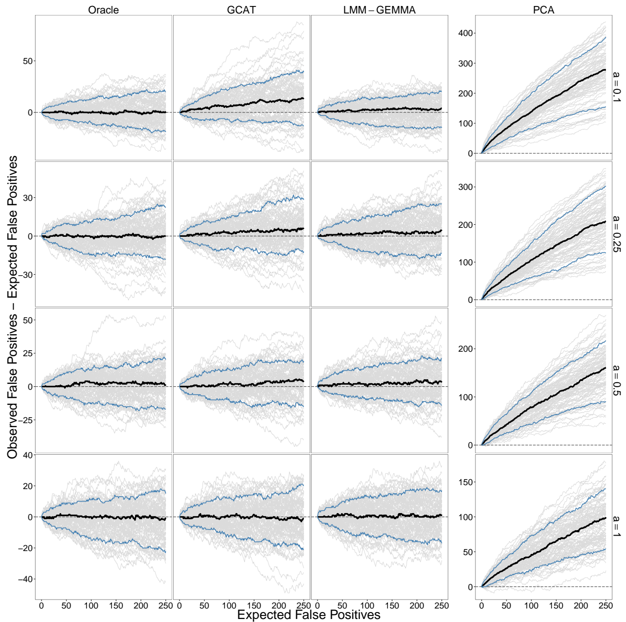
Figure S2: Performance of association tests on 100 simulated studies based off the spatial model of structure for various a comparing the Oracle, GCAT (proposed), LMM (GEMMA), and PCA tests. The variance contributions to the trait are genetic=5%, environmental=5%, and noise=90%. The remaining details are equivalent to Figure 2.
