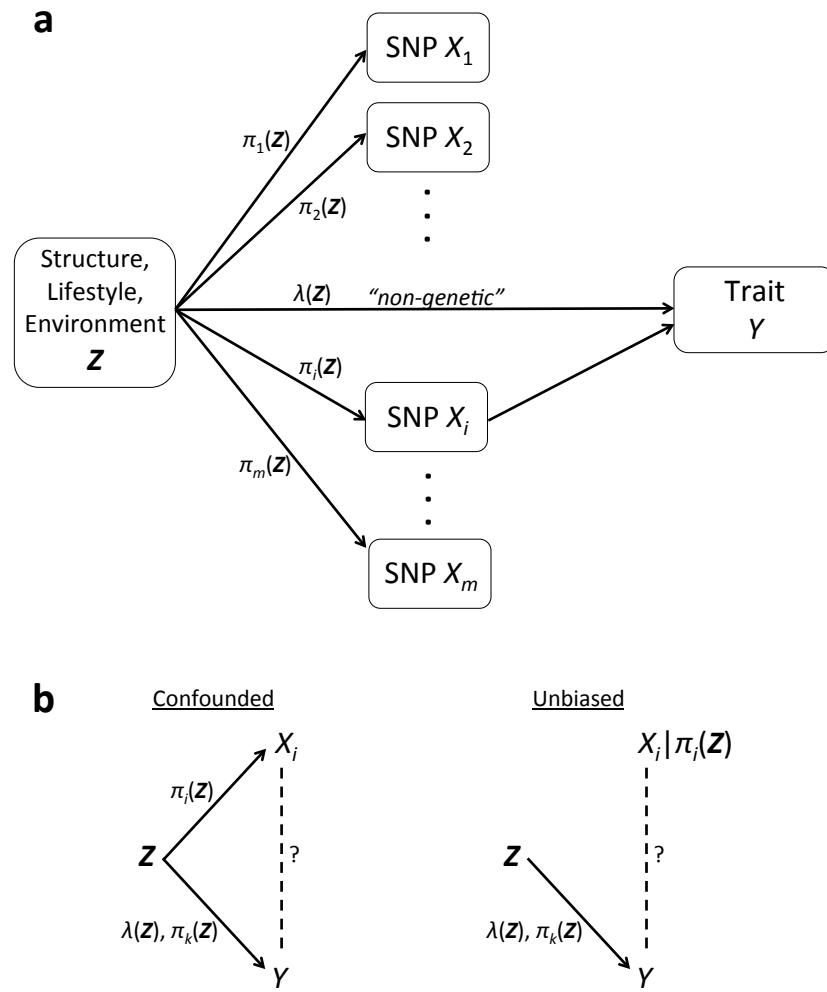
Figure 1: Rationale for the proposed test of association. (a) A graphical model describing population structure and its effects on traits. Population structure serves as a latent causal variable common among a set of loci, via the allele frequencies. When one locus has a causal effect on the trait, this induces spurious associations with other loci affected by population structure. At the same time, population structure may be highly related to lifestyle and the environment as these are all possibly related to ancestry and geography. (b) Accounting for confounding due to latent population structure. Left panel: A test for association between the i th SNP X_i and trait Y without taking into account Z will produce a spurious association due to the fact that both X_i and Y are confounded with Z . Right panel: A test for association between X_i | \pi_i(Z) and Y will be an unbiased because condition on \pi_i(Z) breaks the relationship between Z and X_i .
