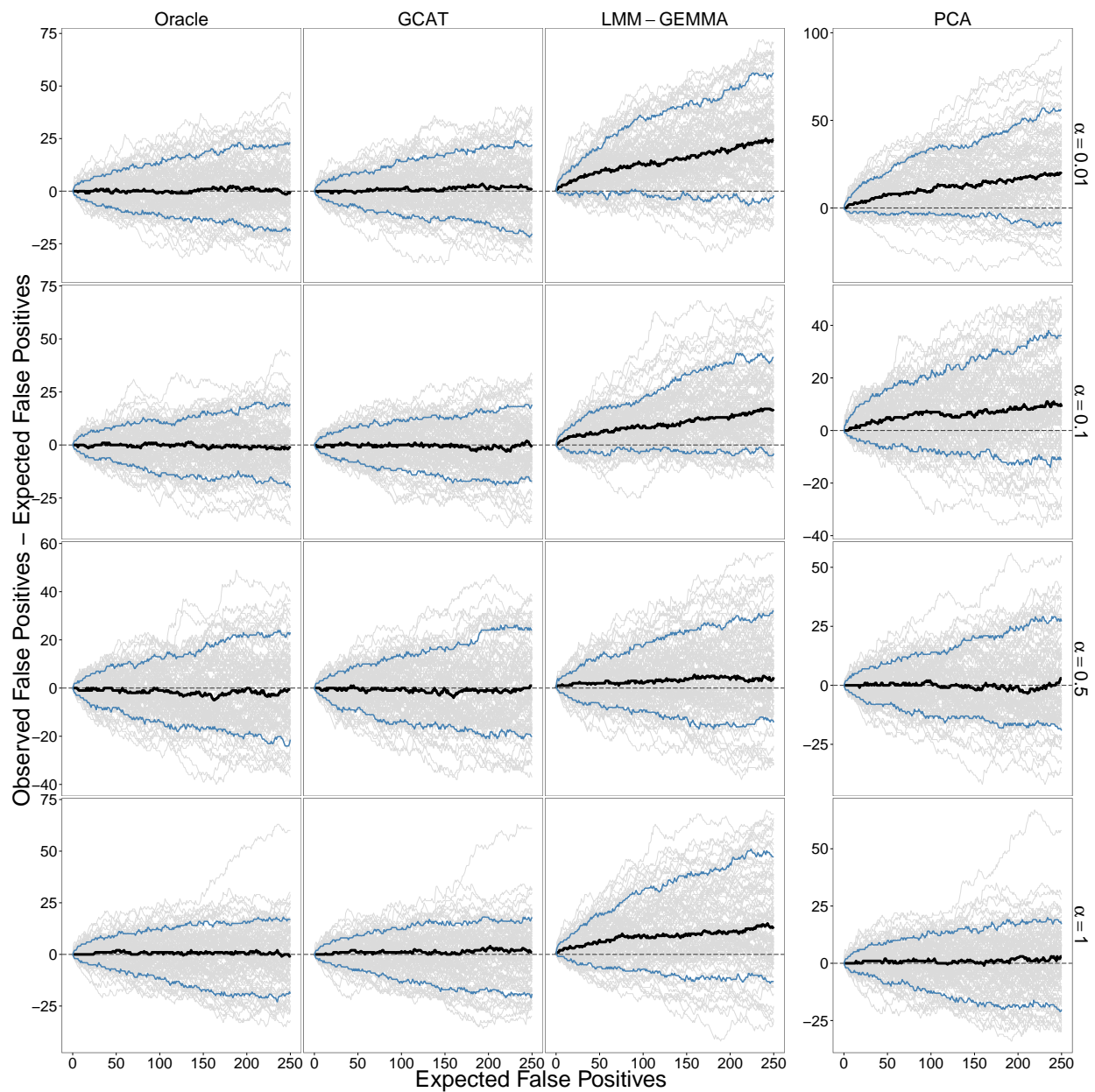
Figure S3: Performance of association tests on 100 simulated studies based off the PSD model of structure for various \alpha comparing the Oracle, GCAT (proposed), LMM (GEMMA), and PCA tests. The variance contributions to the trait are genetic=10%, environmental=0%, and noise=90%. The remaining details are equivalent to Figure 2.
