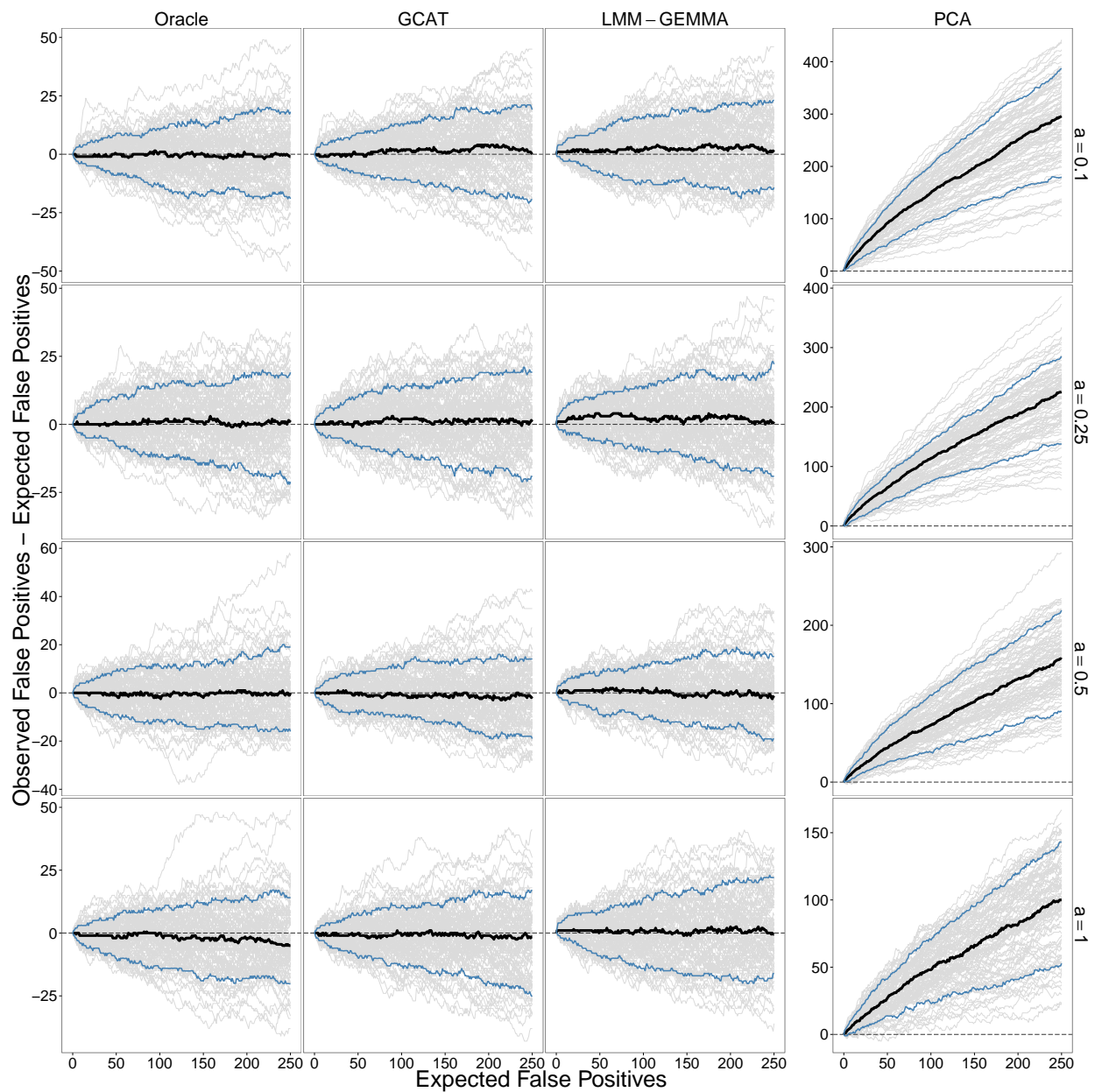
Figure S4: Performance of association tests on 100 simulated studies based off the spatial model of structure for various \alpha comparing the Oracle, GCAT (proposed), LMM (GEMMA), and PCA tests. The variance contributions to the trait are genetic=10%, environmental=0%, and noise=90%. The remaining details are equivalent to Figure 2.
