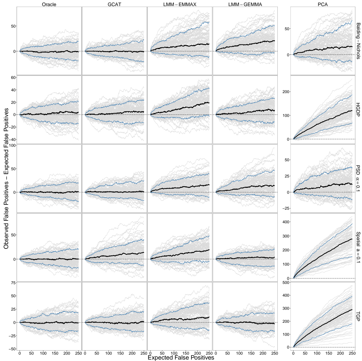
Figure 2: Performance of association tests on 100 simulated studies based off the Balding-Nichols, HGDP, TGP, PSD \alpha = 0.1 , and spatial a = 0.1 simulation scenarios comparing the Oracle, GCAT (proposed), LMM (EMMAX), LMM (GEMMA), and PCA tests. The quantitative traits are based on model (1). The variance contributions to the trait are genetic=5%, environmental=5%, and noise=90%. The differences between the observed number of false positives and expected number of false positives versus the expected number of false positives under the null are plotted for each simulated study (grey lines), the average of those differences (black line), and the middle 90% (blue lines). All simulations had m = 100,000 SNPs, so the range of the x-axis corresponds to choosing a significance threshold of up to 0.0025. The difference on the y-axis is the number of “spurious associations.” PCA is shown on a separate y-axis since it usually has a much larger maximum than the other methods. The Oracle method is where the true allele frequencies are inputted into the proposed test, which we have theoretically proven always corrects for structure.
