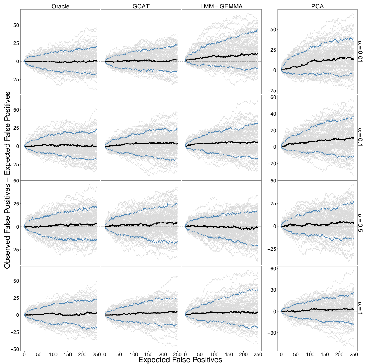
Figure S6: Performance of association tests on 100 simulated studies based off the PSD model of structure for various \alpha comparing the Oracle, GCAT (proposed), LMM (GEMMA), and PCA tests. The variance contributions to the trait are genetic=20%, environmental=10%, and noise=70%. The remaining details are equivalent to Figure 2.
