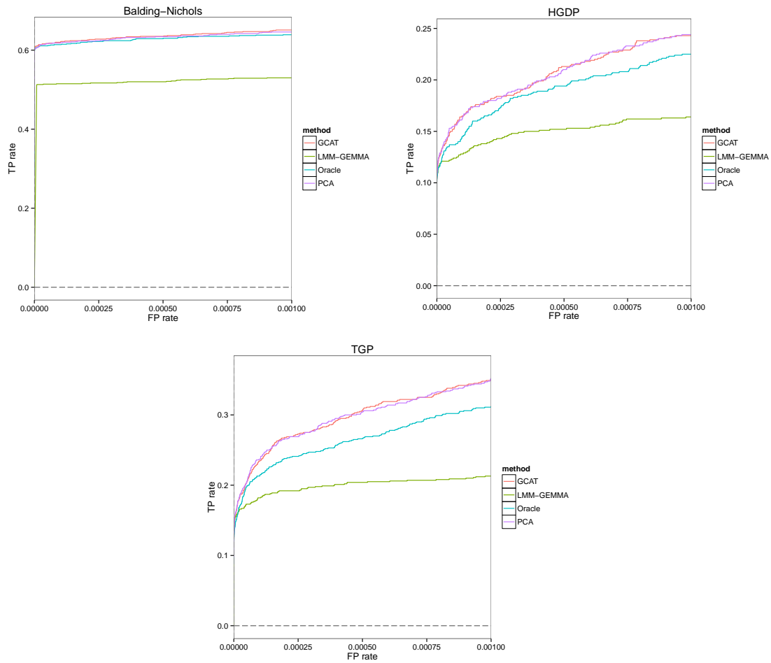
Figure S17: Power analysis for the simulation studies presented in Figure S8.
