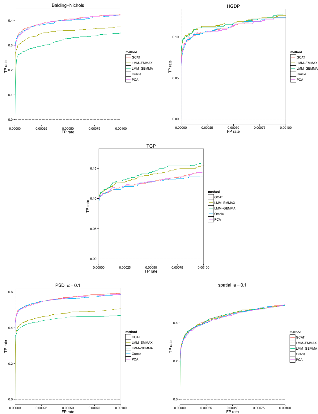
Figure S9: Statistical power of the Oracle, GCAT (proposed), PCA, and both LMM association tests. The results are for the simulated data sets shown in Figures 2. The quantitative traits are based on model (1). The variance contributions to the trait are genetic=5%, environmental=5%, and noise=90%.
