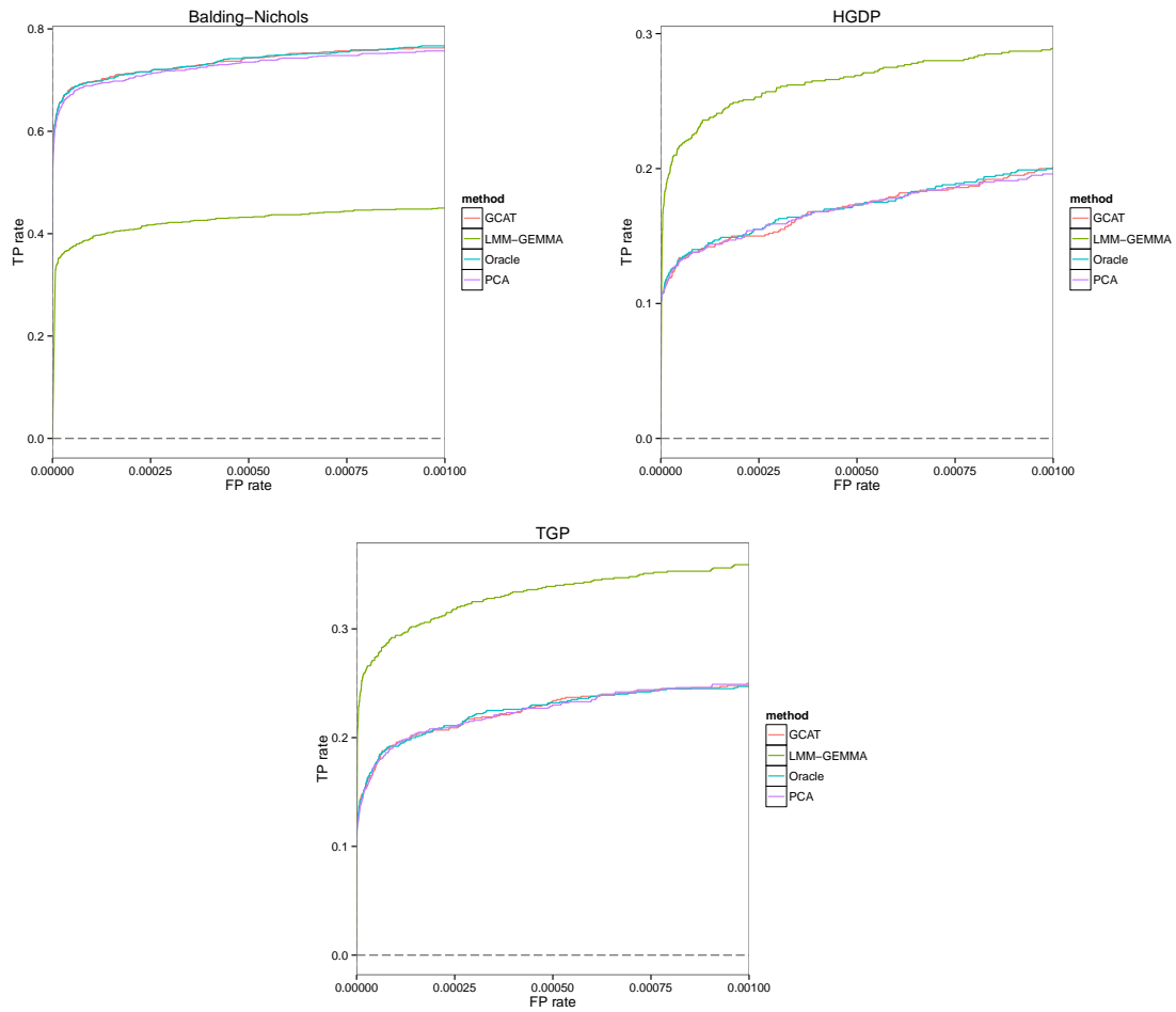
Figure S14: Power analysis for the simulation studies presented in Figure S5.
