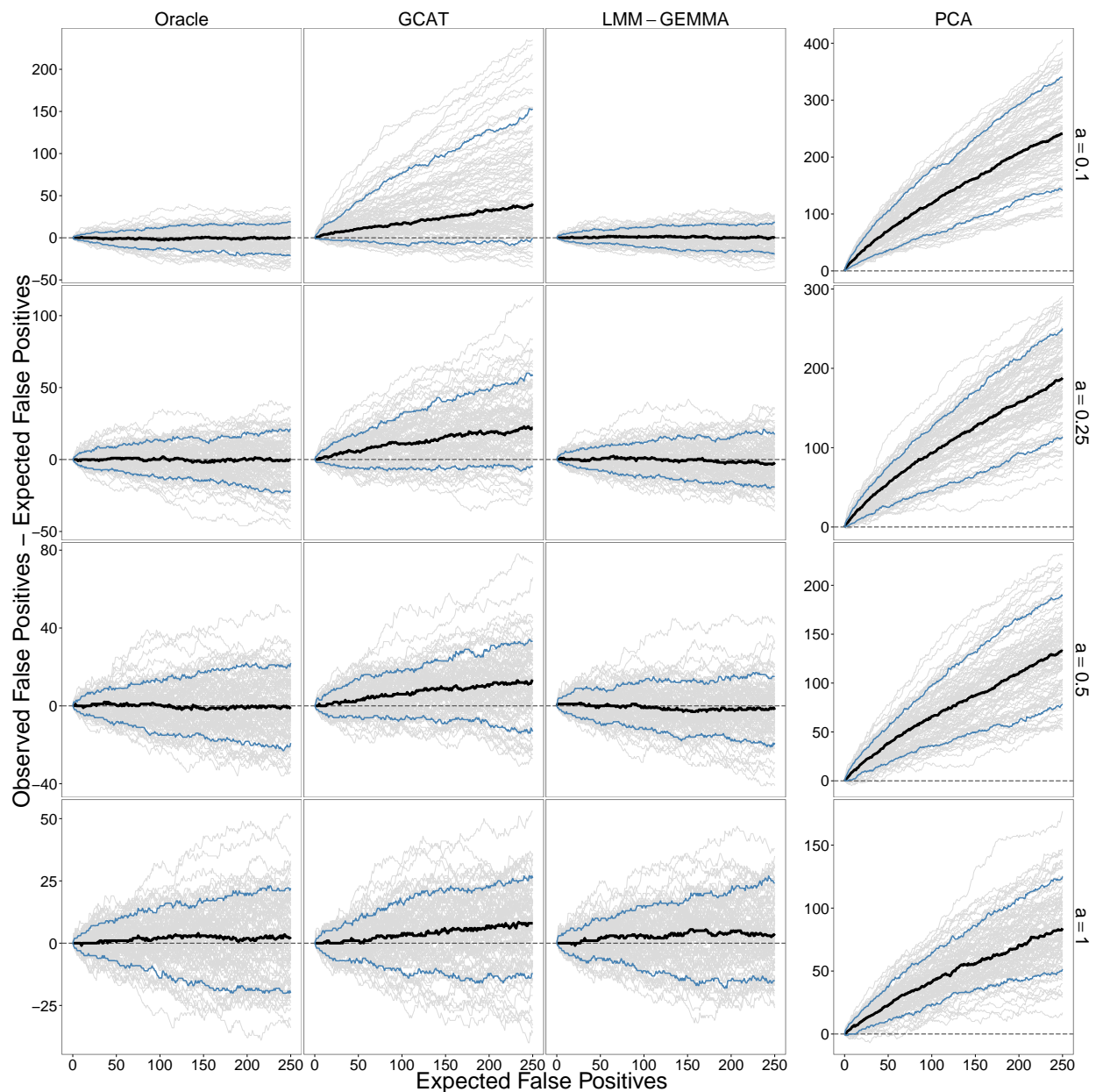
Figure S7: Performance of association tests on 100 simulated studies based off the spatial model of structure for various \alpha comparing the Oracle, GCAT (proposed), LMM (GEMMA), and PCA tests. The variance contributions to the trait are genetic=20%, environmental=10%, and noise=70%. The remaining details are equivalent to Figure 2.
