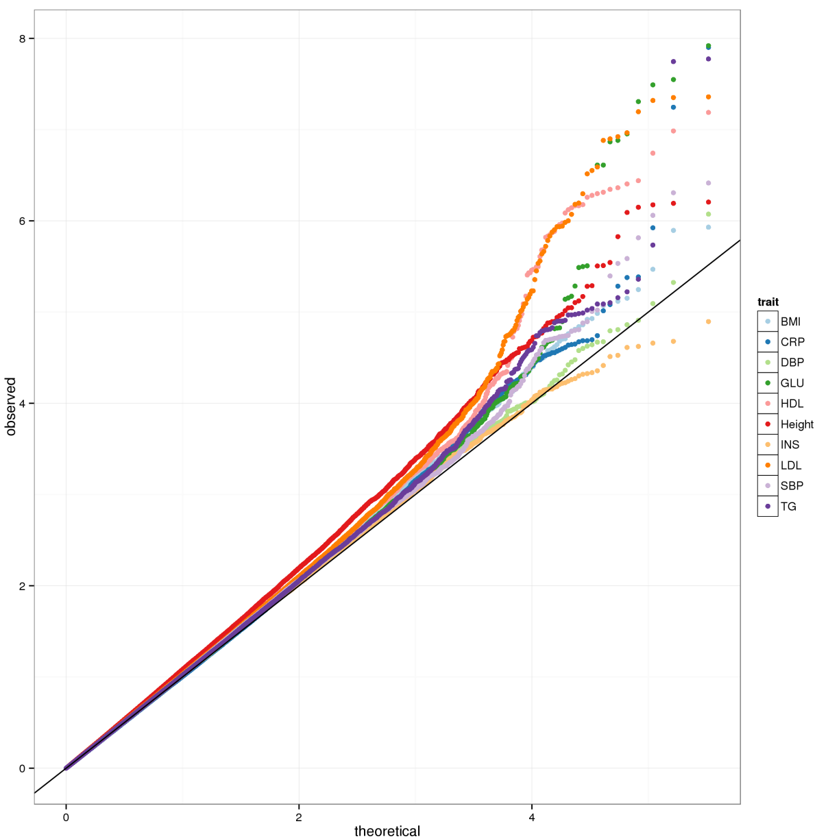
Figure S18: Theoretical versus observed quantiles of -\log_{10}(\text{p-value}) from the GCAT association tests on the Northern Finland Birth Cohort traits. The y-axis was truncated at p-value < 10^{-8} ; see Table S1 for the smallest p-values for each trait.
