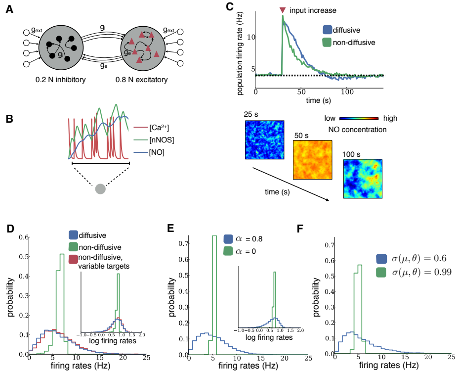
Figure 1. Steady-state behavior of diffusive and non-diffusive homeostasis. (A) Schematic of the sparsely connected recurrent network model. Neurons received homogeneous random spiking input ( g_{ext} ). (B) Intracellular homeostatic signals in a model neuron. Each spike triggers calcium influx, which leads to nNOS activation and NO synthesis. (C) Mean population firing rates for networks with diffusive or non-diffusive homeostasis after an increase in external input (red triangle). Spatial distribution of NO concentrations at different times across the network with diffusion are shown below. (D-F) Distributions of firing rates and log firing rates (insets) after homeostasis from network simulations (D) and mean-field analysis (E), both receiving independent Poisson inputs drawn from a Gaussian distribution. (F) Distributions of firing rates in the mean-field analysis for low and high covariance \sigma of threshold and input rate.
