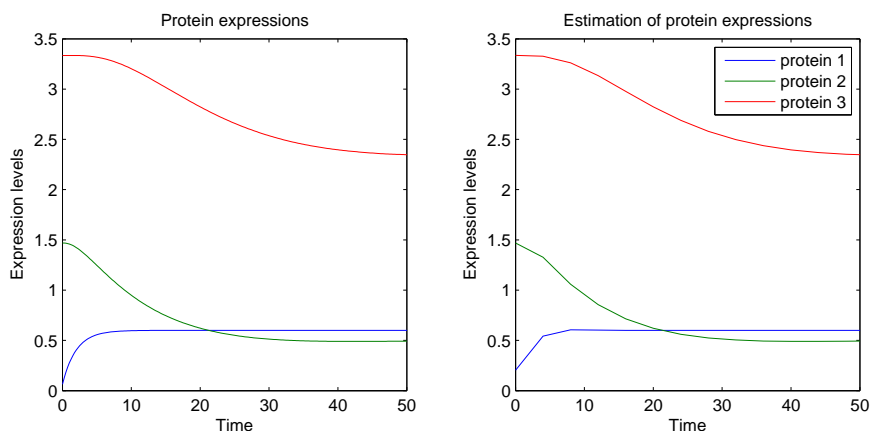
Fig. 6. Exact protein expression curves derived from model ODEs (18) and (19) (left), and their recovered estimations using 12 unnormalized timepoint samples via (P2) (right). For convenience of graphical comparison, the values of r_i were drawn from the system equations. Protein expression is otherwise normalized with respect to r_i , but this would result in a transformed scale for this qualitative comparison.
