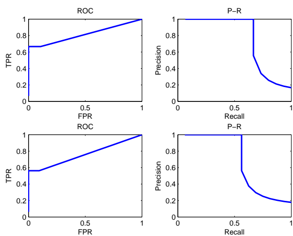
Supplementary Figure 1. ROC and P-R curves for Dream 4, Challenge 2 Network 1 (top) and Network 2 (bottom).
