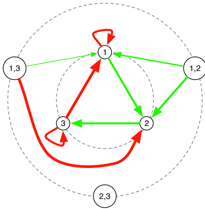
Fig. 4. Map of gene regulatory network described by equations (18) and (19). First-order (single) and second-order (combined) regulators are depicted in concentric circles. Green arrows specify gene activation and red arrows specify gene repression. The relative magnitudes of activation and repression are roughly represented by arrow thickness.
