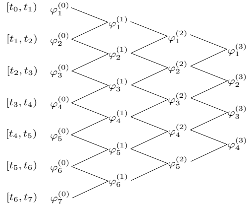
Fig. 8. The De Boor recursion for P = 3 and D = 4 .
