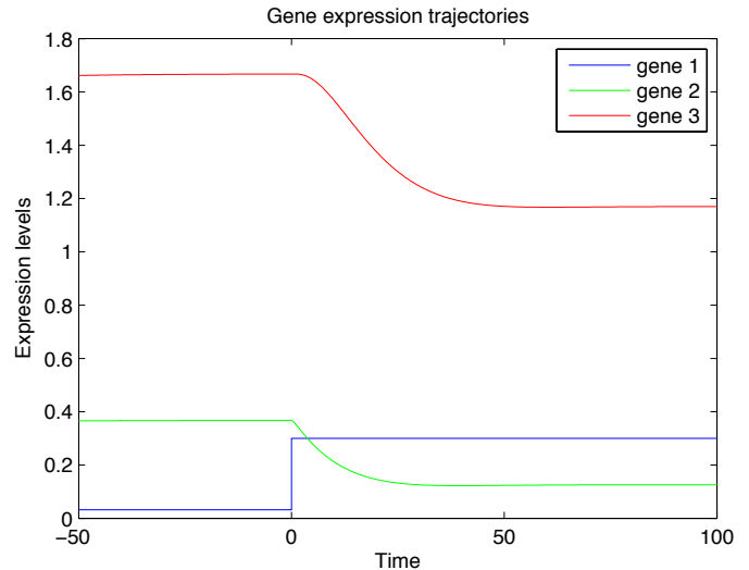
Fig. 5. Gene expression trajectories (unnormalized) before and during the imposed perturbation. The system is in steady state before time 0. Gene 1 is artificially perturbed at time zero, leading to changes in gene expression levels. A new steady state is eventually achieved at approximately time 50. We sample expression levels between time 0 (the starting point of perturbation) and 50 (the new steady state) and use them as data in our algorithm.
