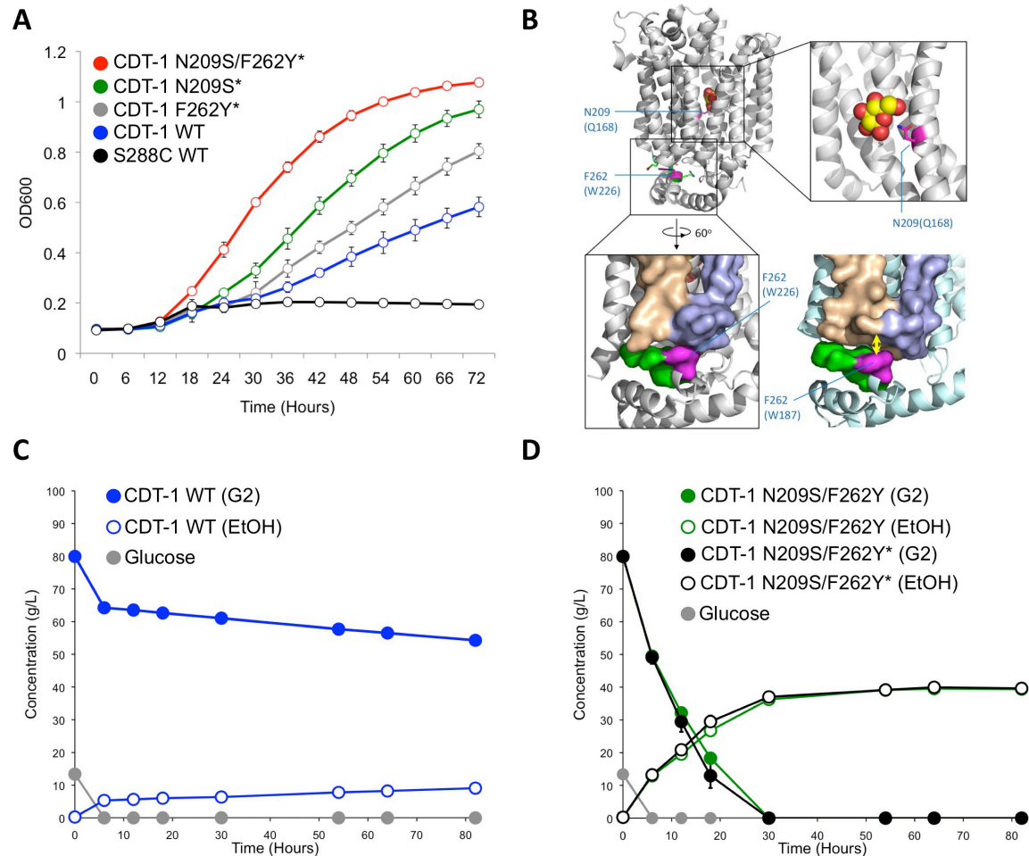
Figure 4. CRISPRm mediated insertion and evolution of chromosomal DNA libraries for in vivo protein engineering. (A) Utilization of cellobiose in CRISPRm-engineered diploid yeast strains. S288C wild type cdt-1 - (black), cdt-1 (blue), cdt-1 Q45H/F262Y/F533Y (indicated as cdt-1 F262Y* on the figure, grey), cdt-1 N209S/I354N/S360P/T406S/W531L (indicated as cdt-1 N209S* on the figure, green) and cdt-1 N209S+Q45H/F262Y/F533Y (indicated as cdt-1 N209S+F262Y* on the figure, red). (B) Location of mutations at conserved sites in the evolved CDT-1 transporter structure. The mutated residues are colored magenta in the top figure, and are mapped onto the E. coli Xyle transporter in the outward-facing configuration bound to glucose (upper panels and lower left, PDB entry 4GBZ), and onto the S. epidermidis GlcP transporter
