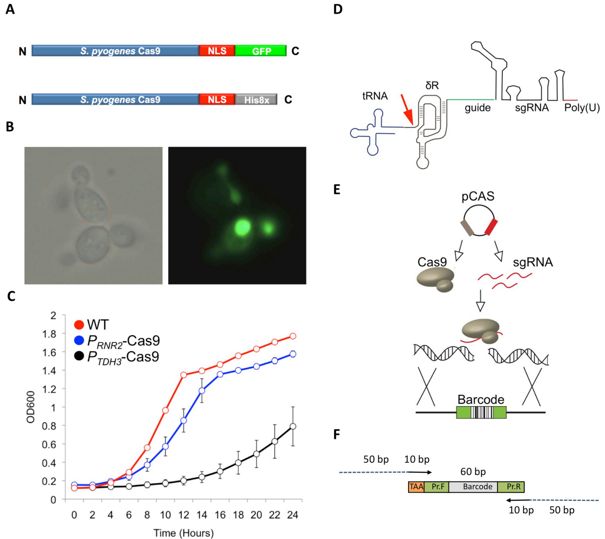
Figure 2. The engineered CRISPRm platform. (A) Cas9 construct used for nuclear localization experiments. The Streptococcus pyogenes Cas9 protein was tagged with a C-terminal nuclear localization motif and a green fluorescent protein (GFP) (green). For genome editing experiments, the Streptococcus pyogenes Cas9 protein was tagged with a C-terminal nuclear localization motif and a Histidine affinity tag (grey). (B) Cellular localization of Cas9-GFP in exponentially growing S. cerevisiae cells. The Cas9-GFP protein was expressed from the TDH3 promoter in this experiment. Left, bright field image; right fluorescence microscopy. (C) Growth
