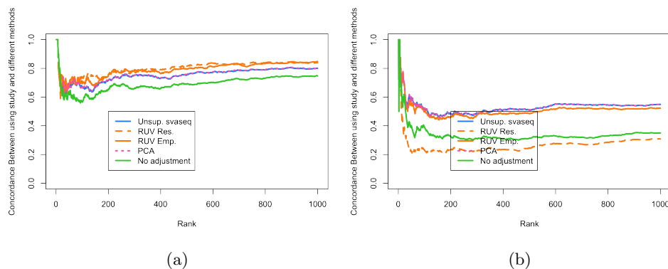
Figure 9: Comparison of differential expression results for ReCount experiment (a) A concordance at the top plot measuring concordance between the analysis using the true study and the various other batch estimates analogous to Figure 6. (b) A concordance at the top plot measuring concordance between the analysis using the true study and the various other batch estimates analogous to Figure 6 when data were resampled to make the sex and study variables moderately correlated ( r^2 = 0.33 .) When sex and study are uncorrelated, RUV performs slightly better and when sex and study are correlated, svaseq performs slightly better. Additional details at http://jtleek.com/svaseq/recount.html
