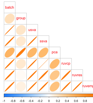
Figure 5: Correlation between simulated batch and group variables and various batch estimates Light circles indicate low correlation and dark, tight ellipses indicate high correlation. In this case, all estimates that respect multiple sources of signal (sva and RUV based) methods are highly correlated with the simulated batch effect. Principal components (sva) estimates a linear combination of the group and batch variable and has lower concordance with the true simulated batch and the other estimates. Additional details at http://jtleek.com/svaseq/simulateData.html .
