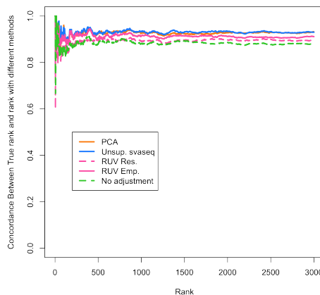
Figure 10: Differential expression results for GEUVADIS data A concordance at the top plot (CAT plot) shows the fraction of DE results that are concordant between the analysis with the true laboratory and the analyses using different batch estimates. Unsupervised surrogate variable analysis for sequencing (blue) and principal components analysis (orange) outperform the RUV based methods (pink) and no batch adjustment (green). Additional details at http://jtleek.com/svaseq/geuvadis.html .
