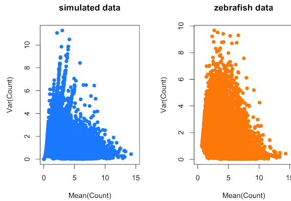
Figure 4: Distribution of means and variances for simulated and real zebrafish data To confirm that my simulation procedure produced reasonable simulated counts, I plotted the gene-specific means and variances for (a) the simulated data set and (b) the observed zebrafish data set. The two distributions are qualitatively similar. Additional checks on the simulation procedure are provided in the simulated data analysis at http://jtleek.com/svaseq/simulateData.html .
