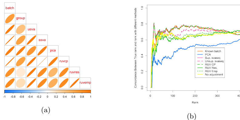
Figure 7: Comparison of batch effect results when group and batch are correlated (a) A plot of the correlation between the different batch estimates and the batch variable analogous to Figure 5. (b) A concordance at the top plot measuring concordance between the analysis using the true batch variable and the various estimates analogous to Figure 6. Here the unsupervised RUV approaches using empirical control probes and residuals perform worse than no adjustment, because the methods can not distinguish signal from the known group variable and the unknown batch variable. Additional details at http://jtleek.com/svaseq/simulateData.html .
