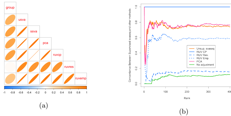
Figure 8: Comparison of batch effect results on zebrafish data (a) A plot of the correlation between the different batch estimates analogous to Figure 5, but with no gold standard. (b) A concordance at the top plot measuring concordance between the analysis using the supervised SVA estimates and the various other batch estimates analogous to Figure 6. The control probes RUV approach (blue solid in (b)) and supervised sva approach produce identical results. The unsupervised sva (orange solid) and principal components (pink solid) approaches are most similar to the supervised estimates in this scenario. Additional details at http://jtleek.com/svaseq/zebrafish.html .
