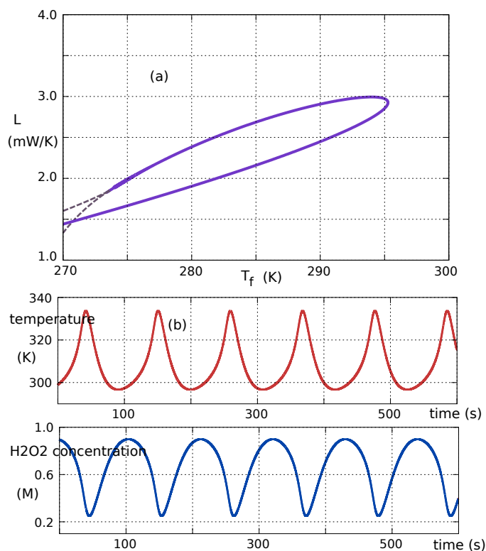
Figure 2. Computed data from equations (1)–(3): (a) Hopf (solid line) and saddle-node (dashed line) bifurcation loci; (b) Time series for T_f = 282 K, L = 2.4 mW; the oscillation period is 108.7 s. (Online version in colour.)
