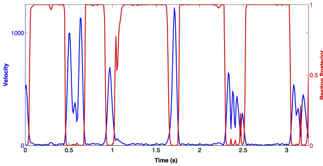
FIG. 17. A typical dynamical sequence in the embedded space. The blue line shows quick bursts of velocity, followed by longer slow periods. The red line shows the posterior probability of belonging to the left-most distribution in Figure 2D.
