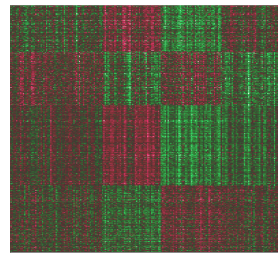
(8) pcNormal48
