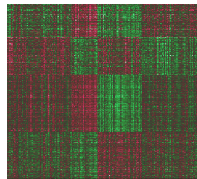
(5) pcNormal43
