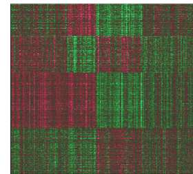
(6) pcNormal44
