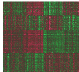
(4) pcNormal42
