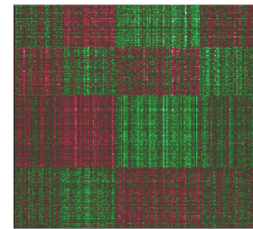
(9) pcNormal50
