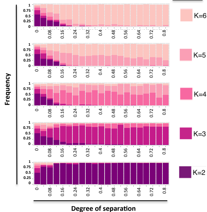
c) CLEST
