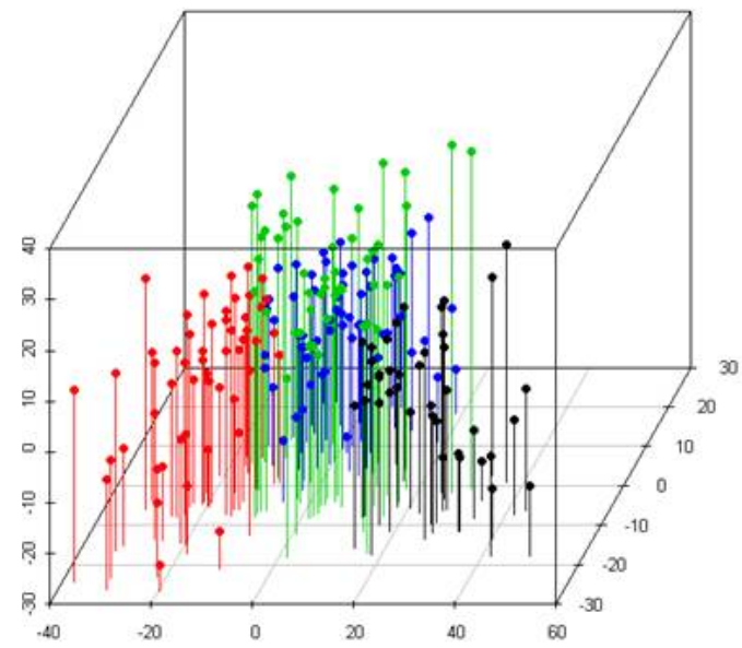
d) First three PCs
