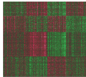
(7) pcNormal45
