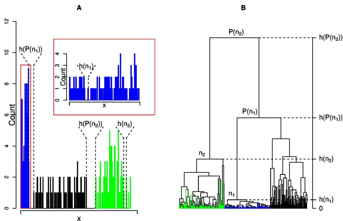
Fig. 1. Tightness analysis for a data set of 280 positive real values sampled from a mixture of three normal components: N(0.5, 0.4^2) ; (blue), N(11, 1^2) ; (green) and N(5, 2^2) . (black). A) A histogram of the data. The inset is an enlarged portion of the histogram enclosed in the red frame B) A hierarchical tree of the data, grown using the absolute difference of the data values as the dissimilarity measure, and single linkage. Thus, the node heights shown in (B) are equal to the corresponding gaps in the data, as indicated in (A) .
