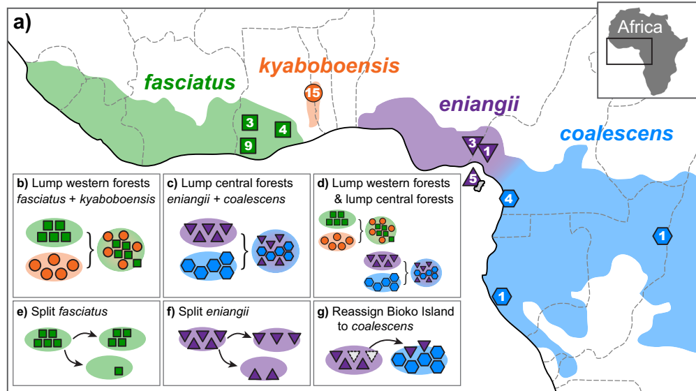
Figure 2: Geographic sampling of Hemidactylus fasciatus complex geckos (numbers in symbols indicate sample sizes), and our preferred current taxonomy (a). BFD* is used to test the alternative species delimitation models outlined in b-g
